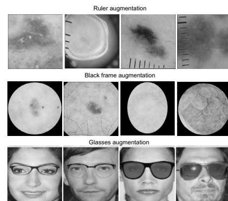
Fig. 2. Example augmentations.
