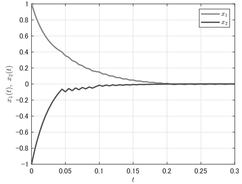
Fig. 1. State trajectories of the SUNLS in Example 1.
