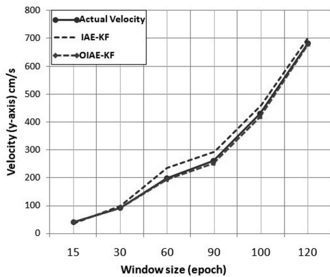
Fig. 10. Estimation analysis between the IAE-KF and the OIAE-KF for the velocity along the y -axis.
