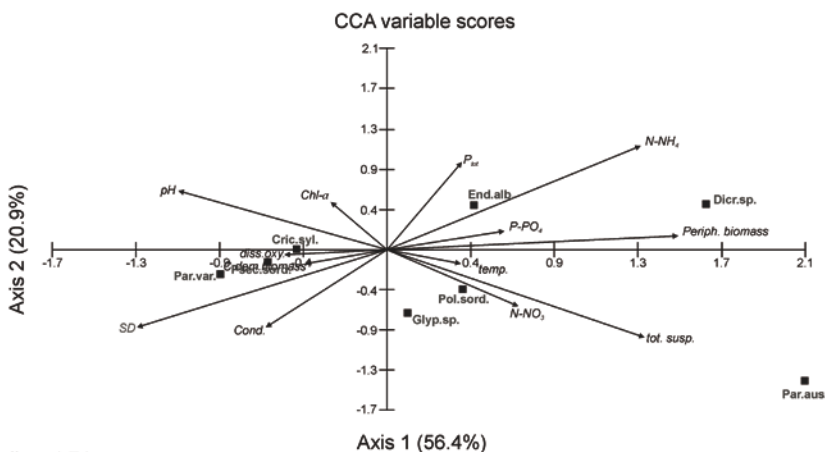
Fig. 2. Canonical Correspondence Analysis (CCA) ordination diagram showing the relation between abundance of midges taxa and environmental variables (temp. - water temperature, SD-Secchi disc depth, cond.-conductivity, tot.susp.-total suspension, N-NH_4 - ammonium nitrogen, N-NO_3 -nitrate nitrogen, Ptot.- total phosphorous, P-PO_4 - orthophosphates, chl-a-epiphytic chlorophyll-a, diss.oxy.-dissolved oxygen, C.dem.biomass-biomass of C. demersum , periph. biomass-biomass of periphyton; Abl.pha.- Ablabesmyia phatta , Clad.man.- Cladotanytarsus mancus , Cric.syl.- Cricotopus sylvestris , Dicr.sp.- Dicrotendipes sp., End.alb.- Endochironomus albigennis , Glyp.sp.- Glyptotendipes sp., Micr.ped.- Microtendipes pedellus , Par.var.- Parachironomus varus , Par.aus.- Paratanytarsus austriacus , Pha.fla.- Phaenopsectra flavipes , Pol.sord.- Polypedilum sordens , Psec.sord.- Psectrocladius sordidellus , Tanyt.sp.- Tanytarsus sp.)
