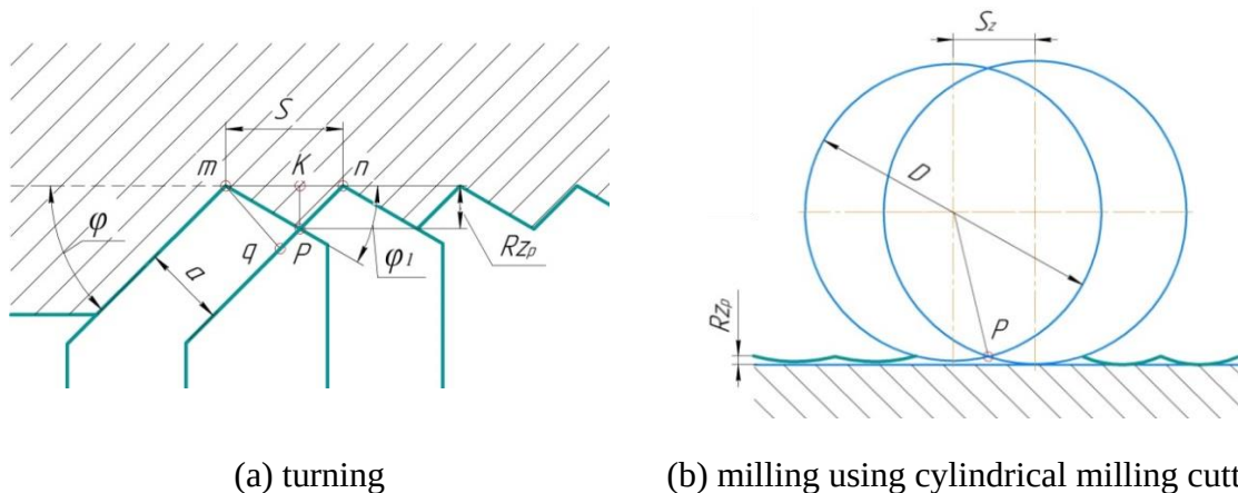
Fig. 1 Theoretical microprofile of the machined surface during turning (a) and milling with cylindrical cutters (b)
