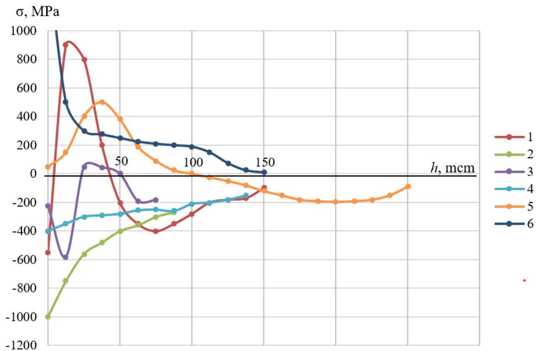
Fig. 5 Distribution of residual stresses along the depth of the surface layer
