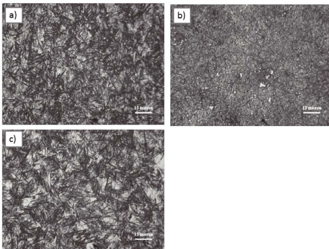
Figure 5. The microstructure of the drill bit (the same magnification): a) A, b) B, c) C
