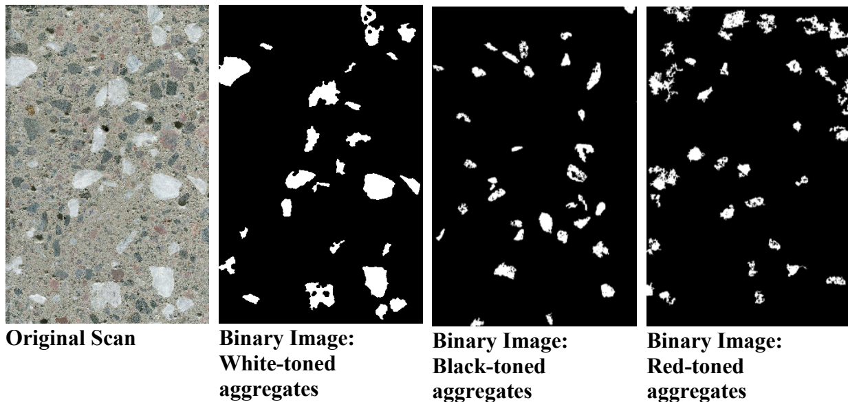
Figure 2 – Original scan of a concrete horizontal slice and its corresponding binary masks highlighting white-toned, red-toned, and black-toned aggregates larger than 5 mm.
