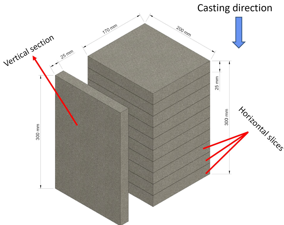
Figure 1 – Schematic representation of the sawn sections in a hardened P-specimen with the casting direction highlighted with the downwards arrow.
