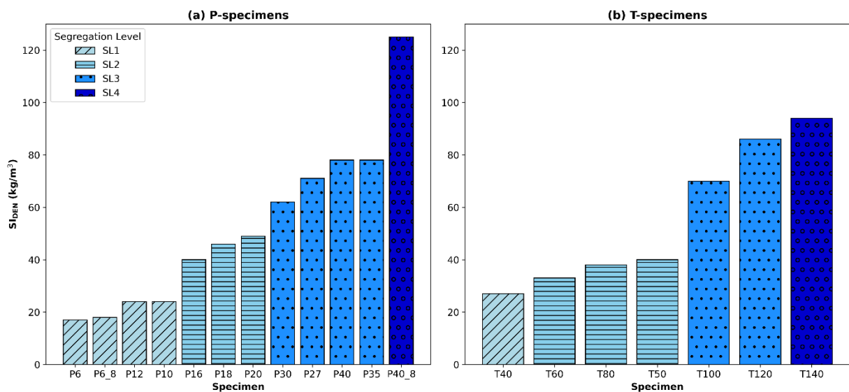
Figure 5 – Standard deviation of densities across the ten slices represented as SI_{DEN} and the corresponding segregation levels according to limits in Table 5.
