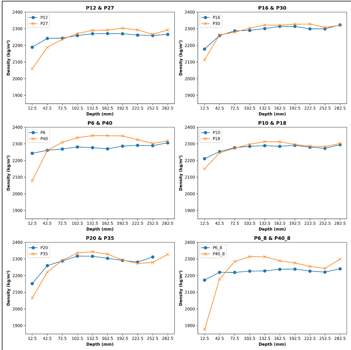
Figure 3 – Density profiles for each pair of poker-vibrated specimens (P-specimens). Note: density at 282.5 mm for P20 is missing due to a broken disc.
