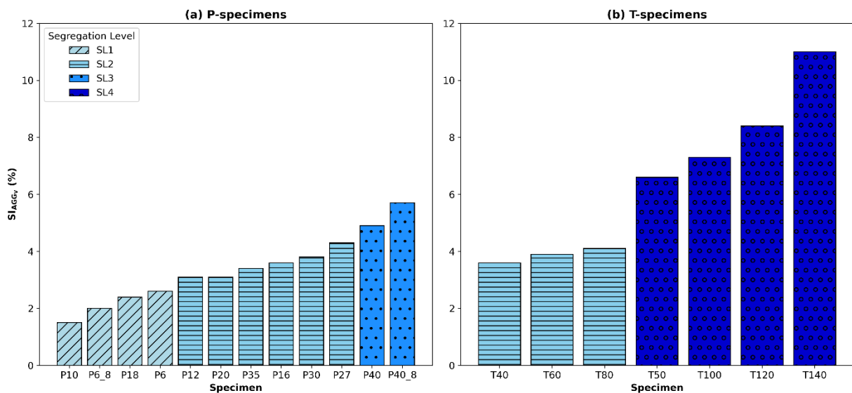
Figure 7 – Standard deviation of aggregate percentages across the ten digitally divided slices of the vertical section represented as SI_{AGG\_V} and the corresponding segregation levels according to limits in Table 6.
