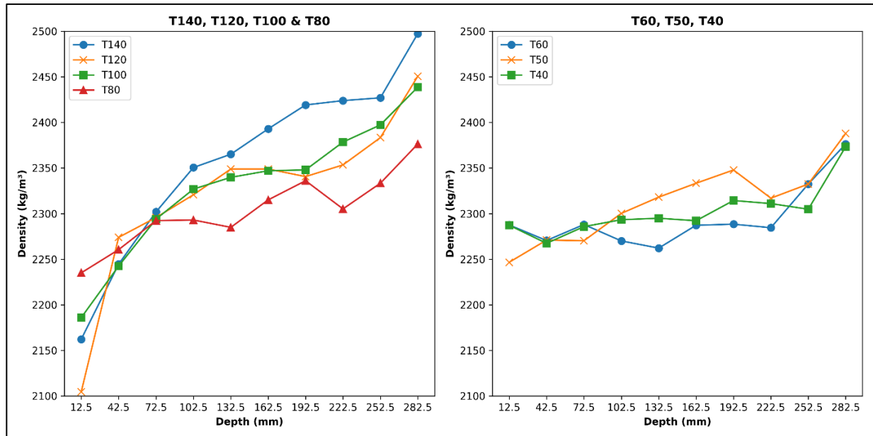
Figure 4 – Density profiles for table-vibrated specimens ( T -specimens).
