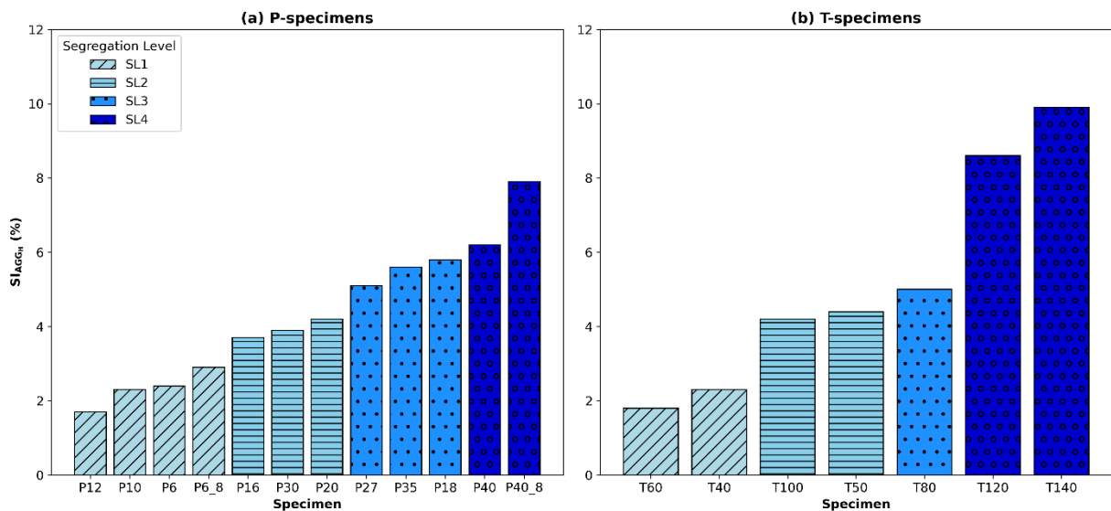
Figure 6 – Standard deviation of aggregate percentages across five slices represented as SI_{AGG\_H} and the corresponding segregation levels according to limits in Table 6.
