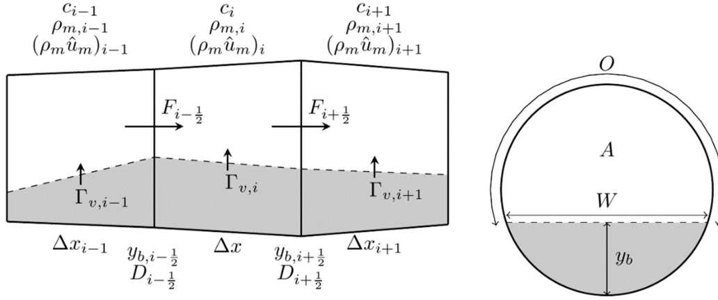
Fig. 2. The grid definition of the 1D-2L Driftflux model. The upper layer represents the flow of sediment and the lower layer the stationary bed. c is the sediment concentration, \rho_m is the mixture density, \Delta x is the cell size, y_b the bed height, D the pipe diameter, F the numerical fluxes, \Gamma_v the bed source term, W the bed width and O the pipe wall surface of the cell portion above the bed.
