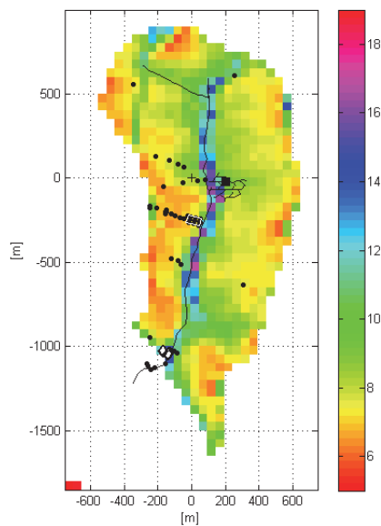
Fig. 4. Topographic index in the Uhlirská catchment; black points – piezometers; black square – piezometer 30; diamonds with white face colour and black edge colour – old ditch, + beginning of coordinates; black full lines – stream and observed ditches; white lines – location of the transect. Remark: The watershed divide at the south of the map is affected by the presence of road.
