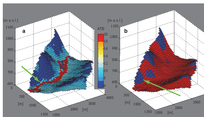
Fig. 7. TOPMODEL predictions of saturated areas (red color) on (a) dry catchment before the major flood 2002 and (b) wet catchment several days after the flood; Jezdecka catchment (4.75 km 2 ); unsaturated cells show the topographic index ATB; predictions conditioned on the mapped pattern of saturation at the site indicated by the arrows (see also Figs. 2 and 6).
