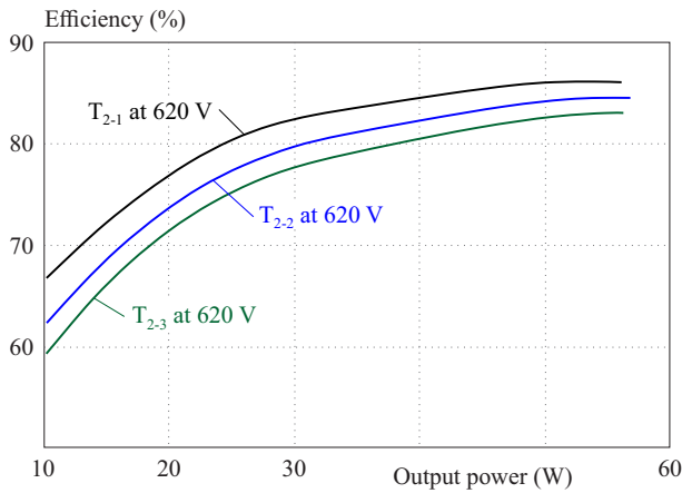
Fig. 15. The 57 W ACF efficiency curves with 620 V input in ACM
