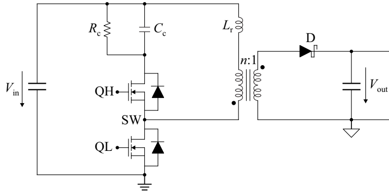
Fig. 2. The ACF generic schematics with resonant inductance
