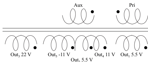
Fig. 3. The schematic symbol of the transformer T2
