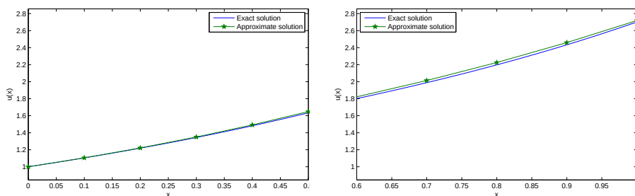
Fig. 3. Comparison of solutions in [0, 0.5] and [0.6, 1]
