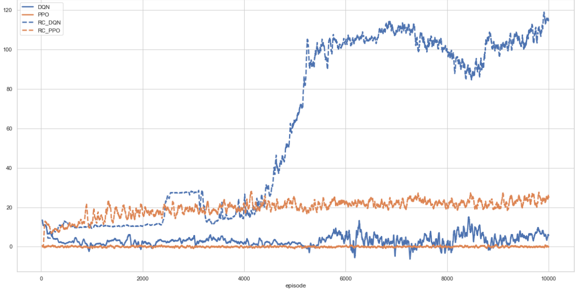
Figure 1: Performance of DQN, PPO, and their reality-checks on an extended environment combining OpenAI gym’s CartPole and our IgnoreRewards. Episode number is plotted on the horizontal axis, and average episode reward is plotted on the vertical axis.
