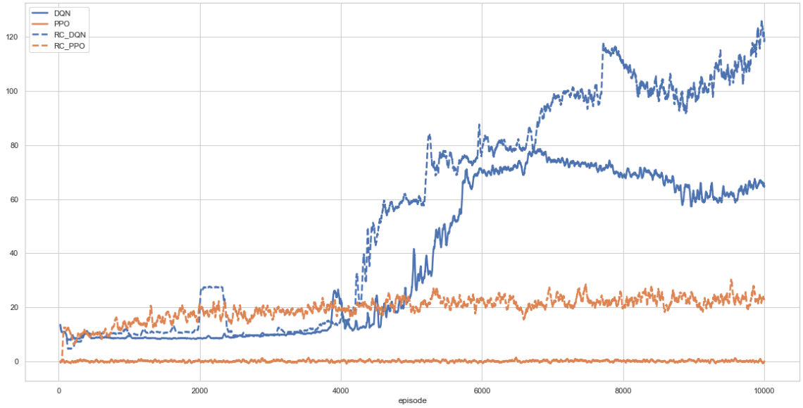
Figure 2: Performance of DQN, PPO, and their reality-checks on an extended environment combining OpenAI gym’s CartPole and our IncentivizeLearningRate. Episode number is plotted on the horizontal axis, and average episode reward is plotted on the vertical axis.
