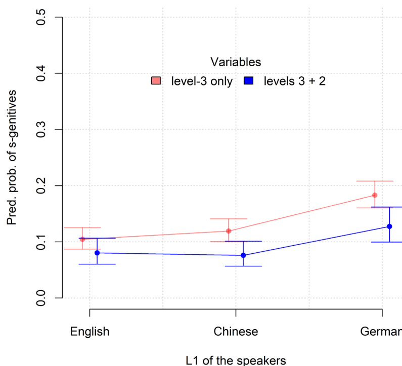
Figure 2. Predicted probabilities of s -genitives (analysis 2).
