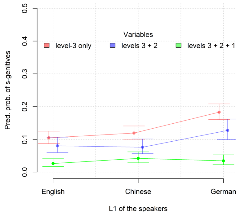
Figure 3. Predicted probabilities of s -genitives (analysis 3a).
