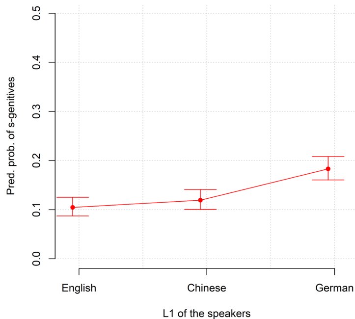
Figure 1. Predicted probabilities of s -genitives (analysis 1).
