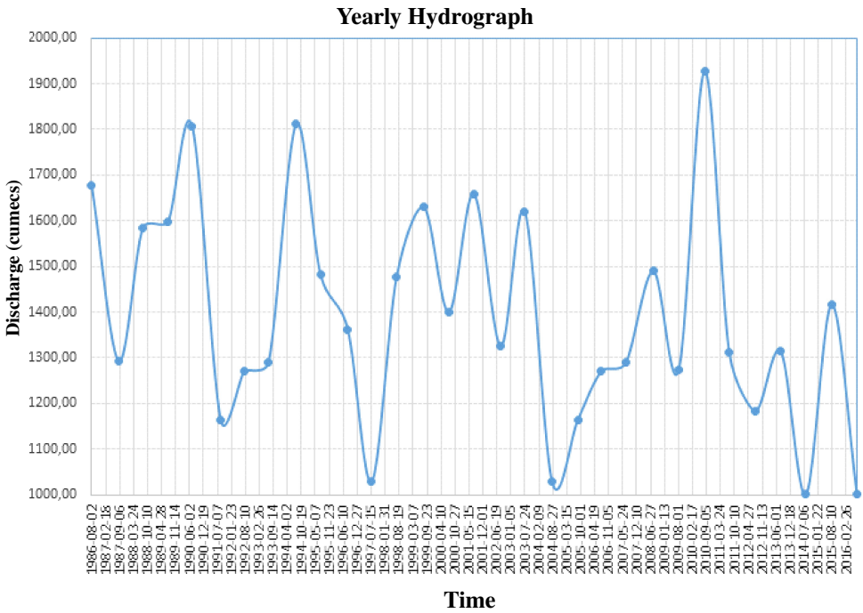
Fig. 7. Runoff Hydrograph
