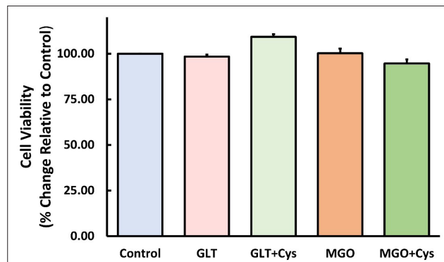
Figure 5. CYS, GLT, and MGO treatment to cells did not affect cell viability
