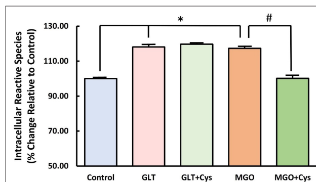
Figure 3. BSA glycation with glucose increased potential AGE formation and is significantly inhibited by CYS
