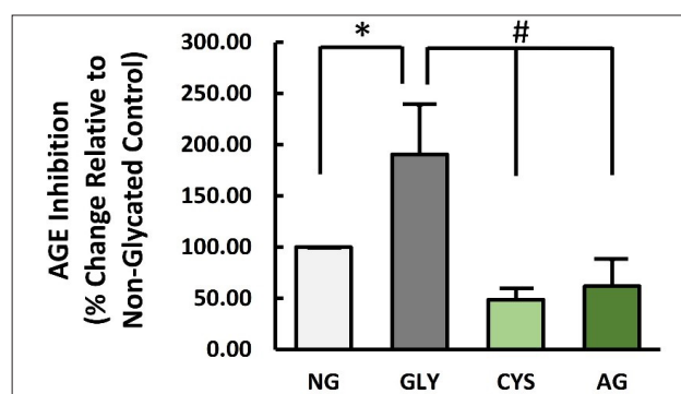
Figure 2. CYS effectively sequesters and prevents methylglyoxal-induced glycation of BSA
