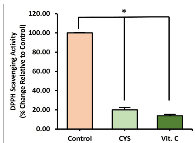
Figure 6. CYS is an effective scavenger of free-radical species. Data are expressed as percentage change relative to control
