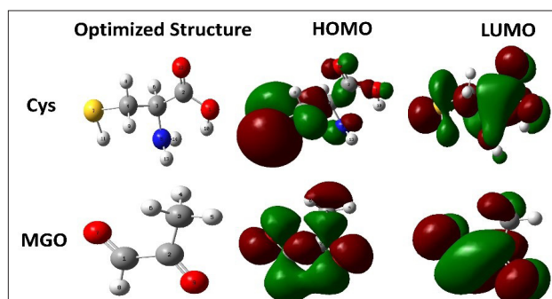
Figure 1. Frontier molecular orbitals of CYS and Methylglyoxal (DFT/B3LYP/6-31G (d))
