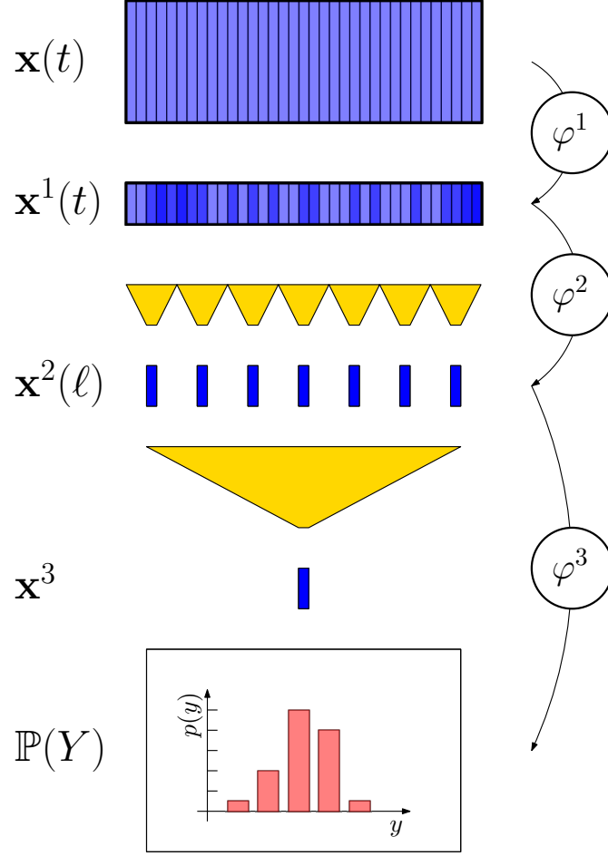
Figure 2. The proposed deep learning system for the analysis of handling properties. The trajectory condenser \varphi^1 reduces the size of each point in the input trajectory (the first blue rectangle); the trajectory analyser \varphi^2 summarises local portions of the driving experience into fewer feature vectors; the trajectory classifier \varphi^3 outputs a probability mass function \mathbb{P}(Y) = (p(y_1), p(y_2), \dots, p(y_{N_y})) over the scores space, representing a global evaluation of the driving experience. Yellow trapezoids represent attention mechanisms.
