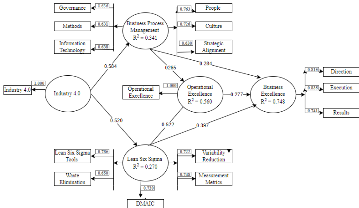
Figure 2 Second-order PLS-SEM model
