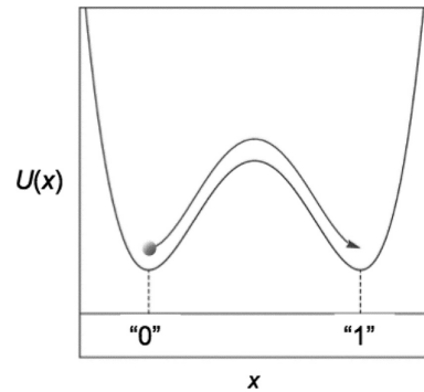
Figure 4. A single-bit storage device.
