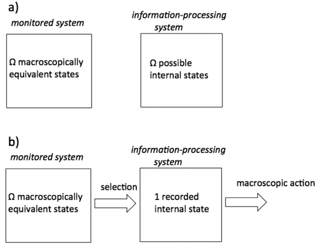
Figure 1. A monitored system and an information-processing system a) before, and b) after the selection process.
