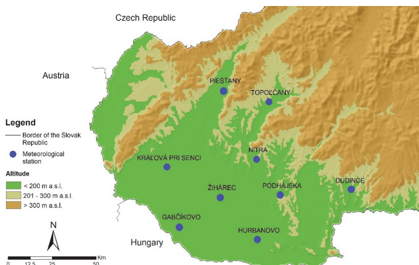
Figure 1 Meteorological stations (Danube Lowland)
