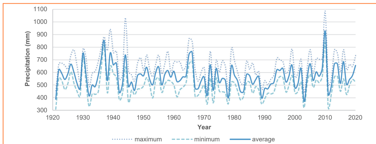
Figure 2 Maximal, minimal, and average precipitation value for the stations in the Danube Lowland (1921–2020)
