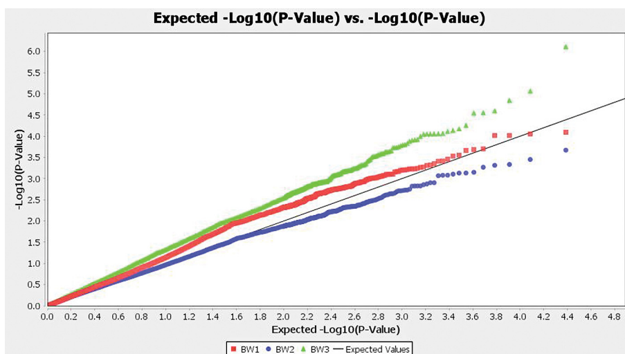
Figure 1. QQ-plots of body weight at one year (BW1), two years (BW2), and three years (BW3) of age in the pooled animals. Dots indicate -\text{Log}_{10}(p) values for individual SNPs. The line indicates the expected values when confirming the null hypothesis of the absence of associations.
