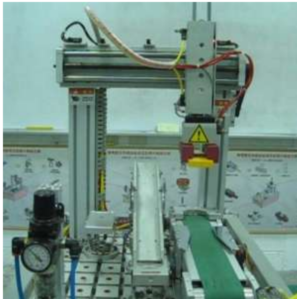
Figure 5. Movement of a rectangular piece (step 1)
