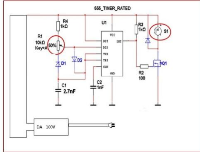
Figure 8. Circuit of light source. The light intensity of the LED source can be adjusted by using a pulse width modulation (PWM) circuit.
