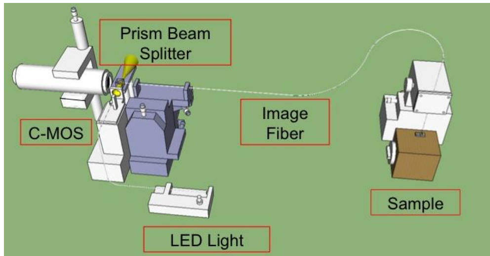
Figure 3. System schematic
