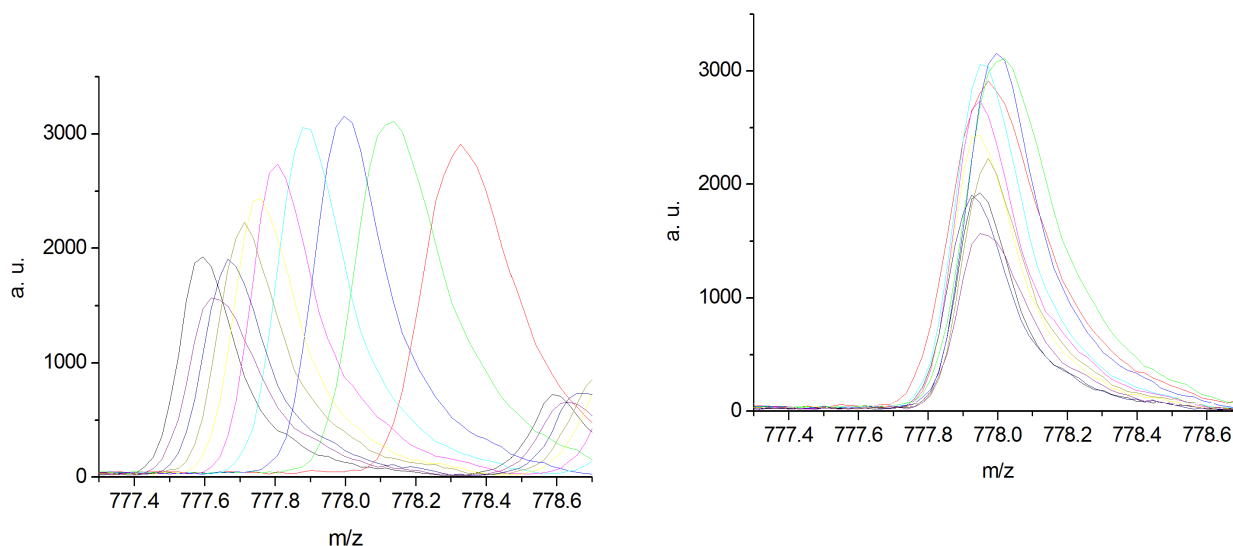
Figure 3 10 replicate LDI-MS spectra of Uniball ink lines on paper 3: (a) shift in the m/z spectra between ink specimens (b) recalibrated data.
