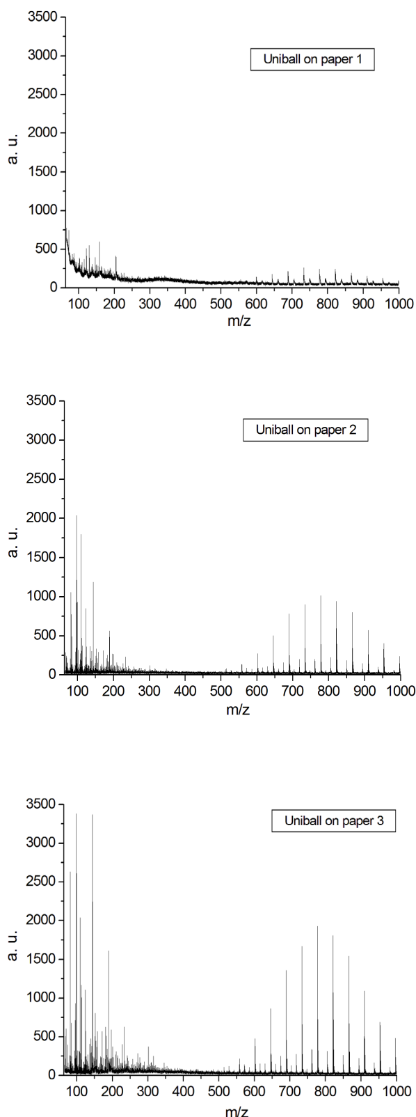
Figure 7 LDI-MS Spectra of Uniball on three papers (recycled), 2 (Xerox) and 3 (HP).
