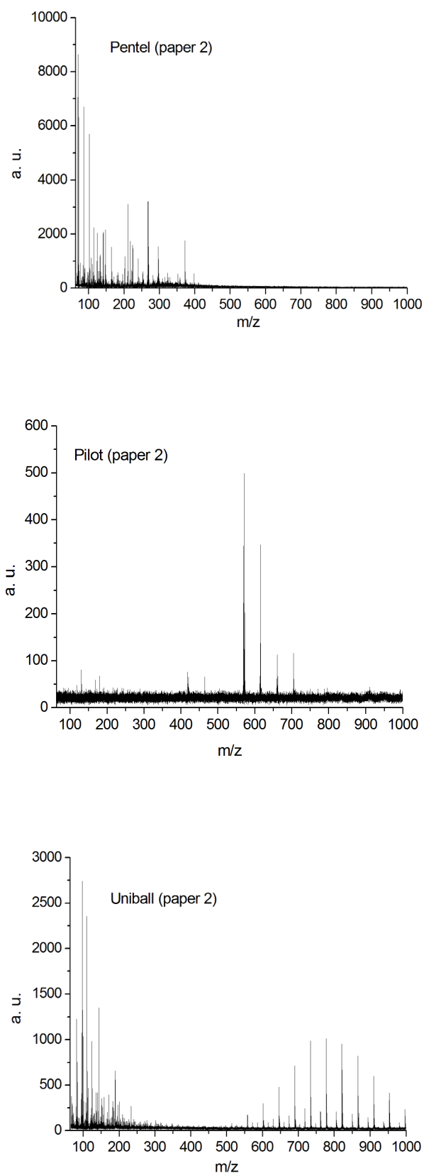
Figure 2 LDI-MS Spectra of gel pen inks: Pentel, Pilot and Uniball on paper 2 (Xerox).
