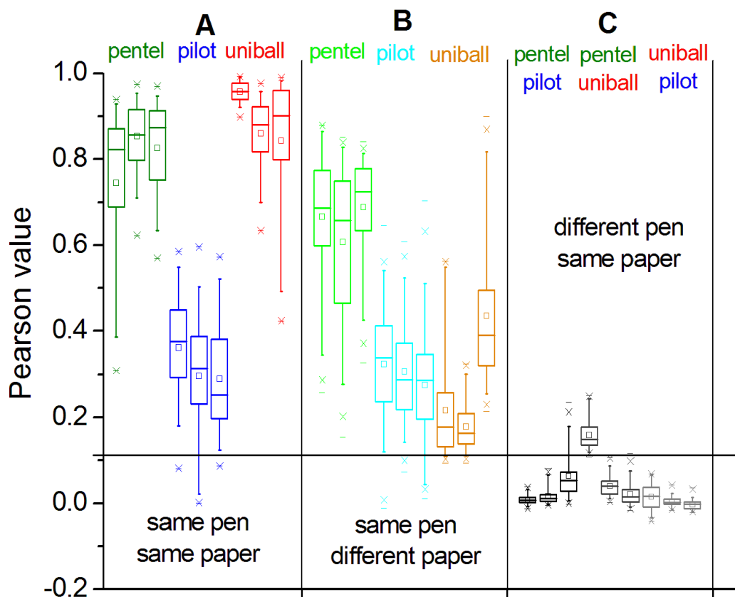
Figure 4 - Box charts showing the distribution of Pearson correlation coefficient values for the comparison of ink samples: (A) same pen on same paper (each set of three boxplots representing within paper 1, 2 and 3 respectively), (B) same pen on different paper (each set of three boxplots representing comparison between paper 1&2, 1&3 and 2&3 respectively), and (C) different pen on the three different paper types (each set of three boxplots representing within paper 1, 2 and 3 respectively).
