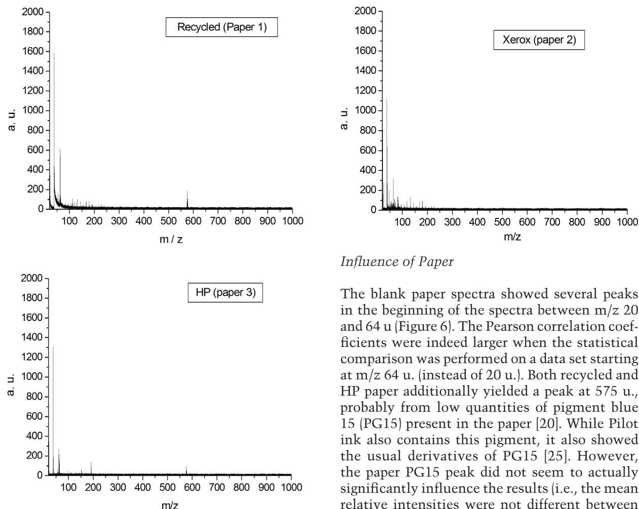
Figure 6 LDI-MS Spectra of blank paper 1 (recycled), 2 (Xerox) and 3 (HP).
