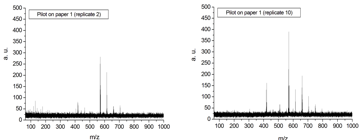
Figure 5 LDI-MS Spectra of gel pens ink Pilot on paper 1: replicate analyses 2 and 10 yielded significantly different spectra (resulting in a low Pearson correlation value of 0.07 for the comparison).
