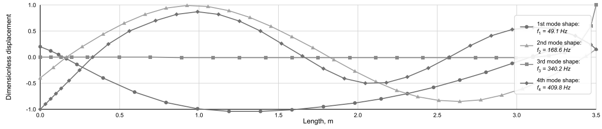
Fig. 10. Mode shapes for eigenfrequencies obtained for the evaluated bearing stiffness parameters using the modified Moore–Penrose pseudoinverse.
