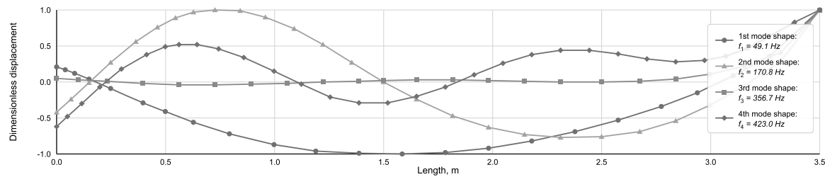
Fig. 16. Mode shapes for eigenfrequencies obtained for the evaluated bearing stiffness parameters using the artificial neural network.
