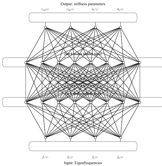
Fig. 11. General neural network architecture.
