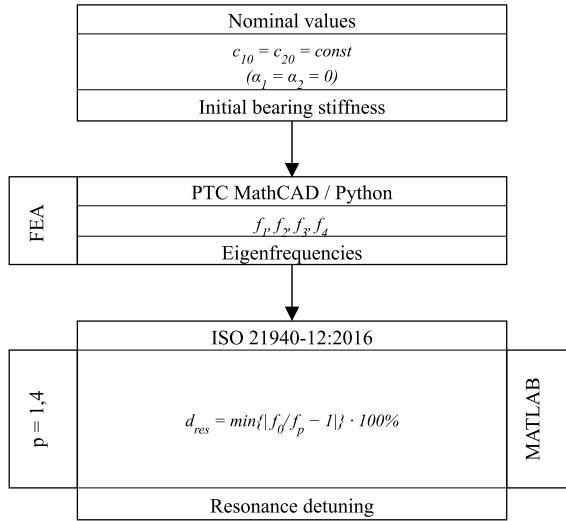
Fig. 2. Finite element analysis of rotor dynamics.
