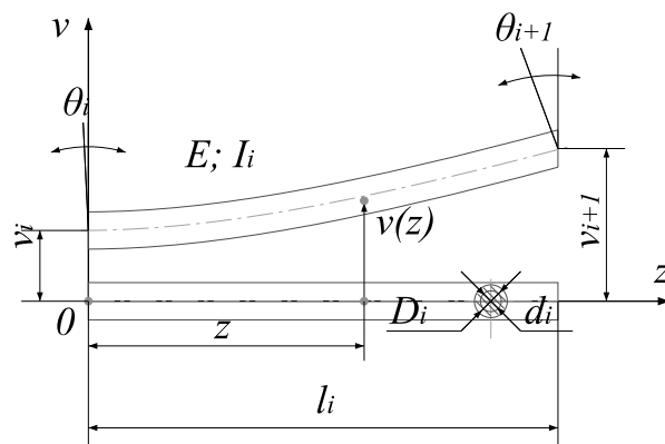
Fig. 1. Design scheme of the finite element.
