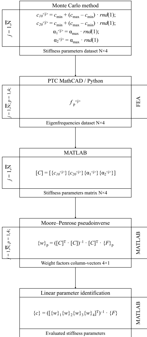
Fig. 3. Linear parameter identification using a modified Moore–Penrose pseudoinverse.
