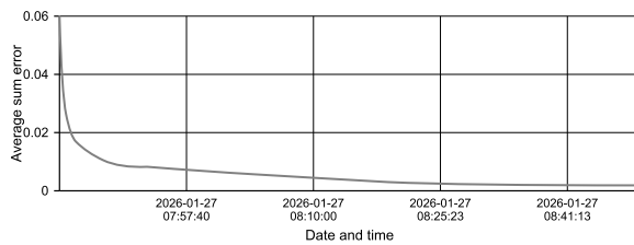
Fig. 14. Training error.
