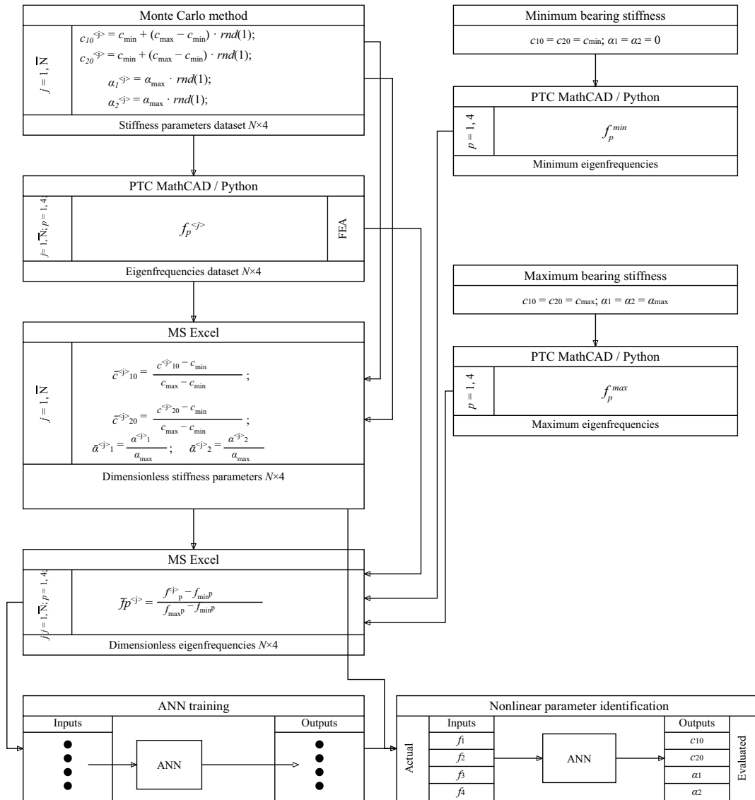
Fig. 6. Nonlinear parameter identification using an artificial neural network.
