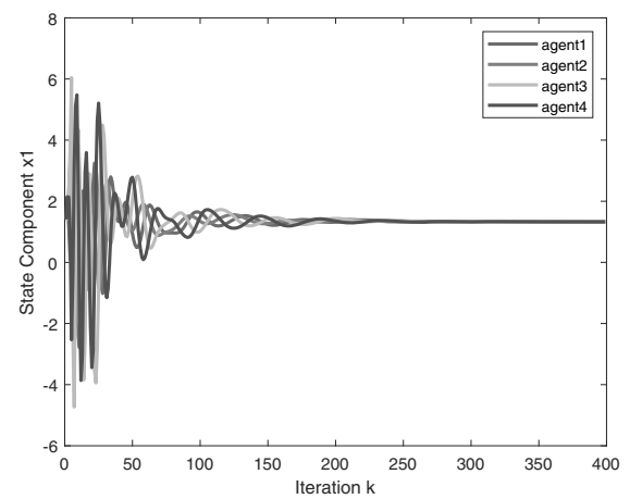
Fig. 11. Variation of the agent's state component 1.
