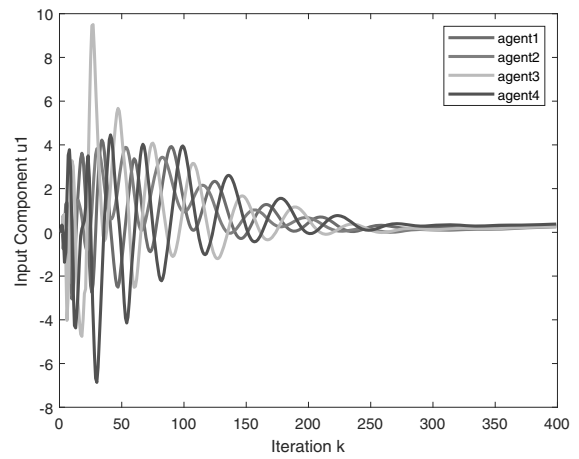
Fig. 10. Variation of the agent's input component 2.
