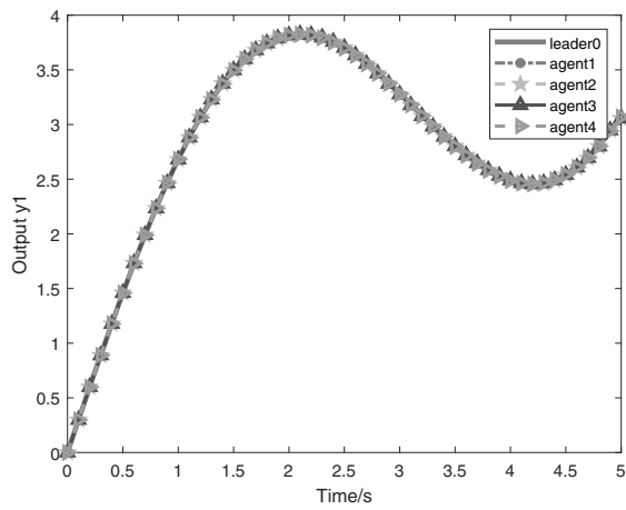
Fig. 7. Output component 2 of agents at the 400th iteration.
