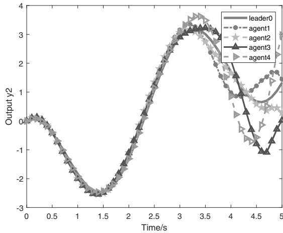
Fig. 4. Output component 2 of agents at the 50th iteration.
