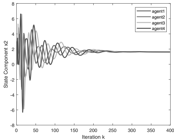
Fig. 12. Variation of the agent's state component 2.
