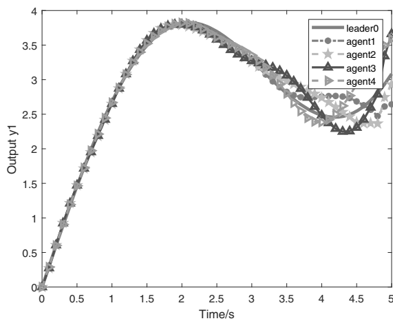
Fig. 5. Output component 1 of agents at the 150th iteration.
