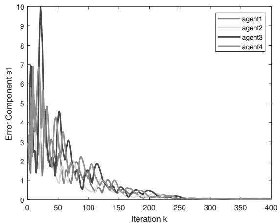
Fig. 13. Variation of the agent's error component 1.
