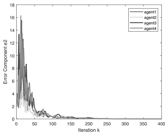
Fig. 14. Variation of the agent's error component 2.
