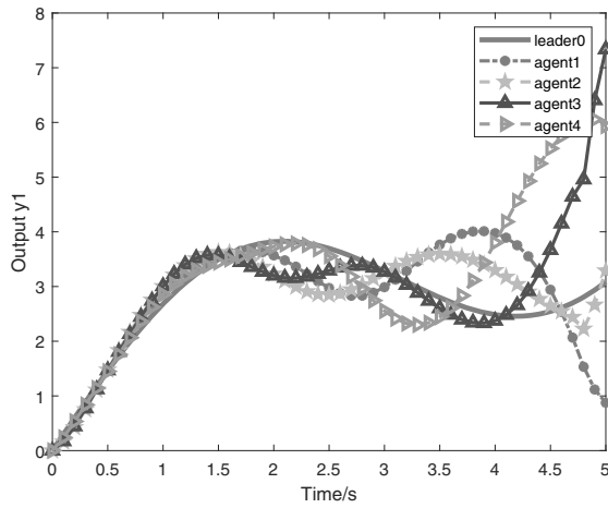
Fig. 3. Output component 1 of agents at the 50th iteration.
