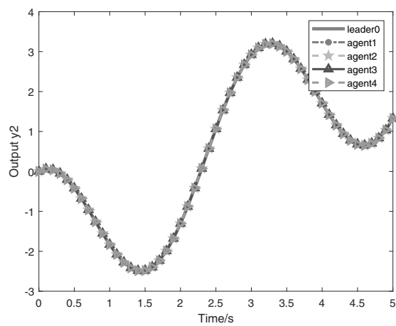
Fig. 8. Output component 2 of agents at the 400th iteration.
