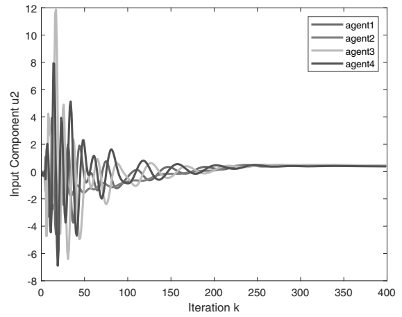
Fig. 9. Variation of the agent's input component 1.
