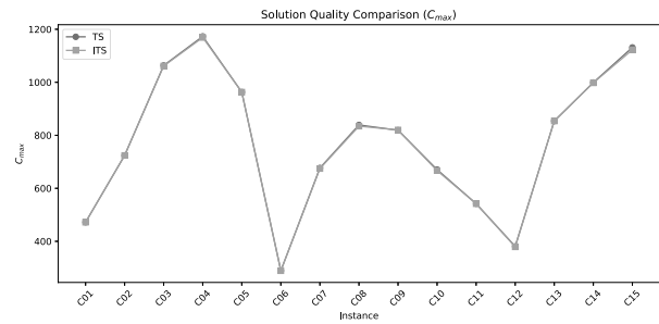
(a) comparison of C_{\max} on medium-scale instances.
