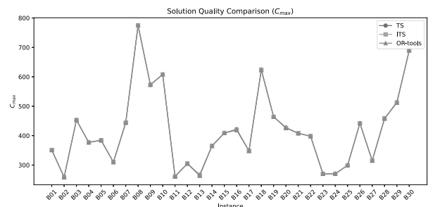
(a) comparison of C_{\max} on small-medium-scale instances.
