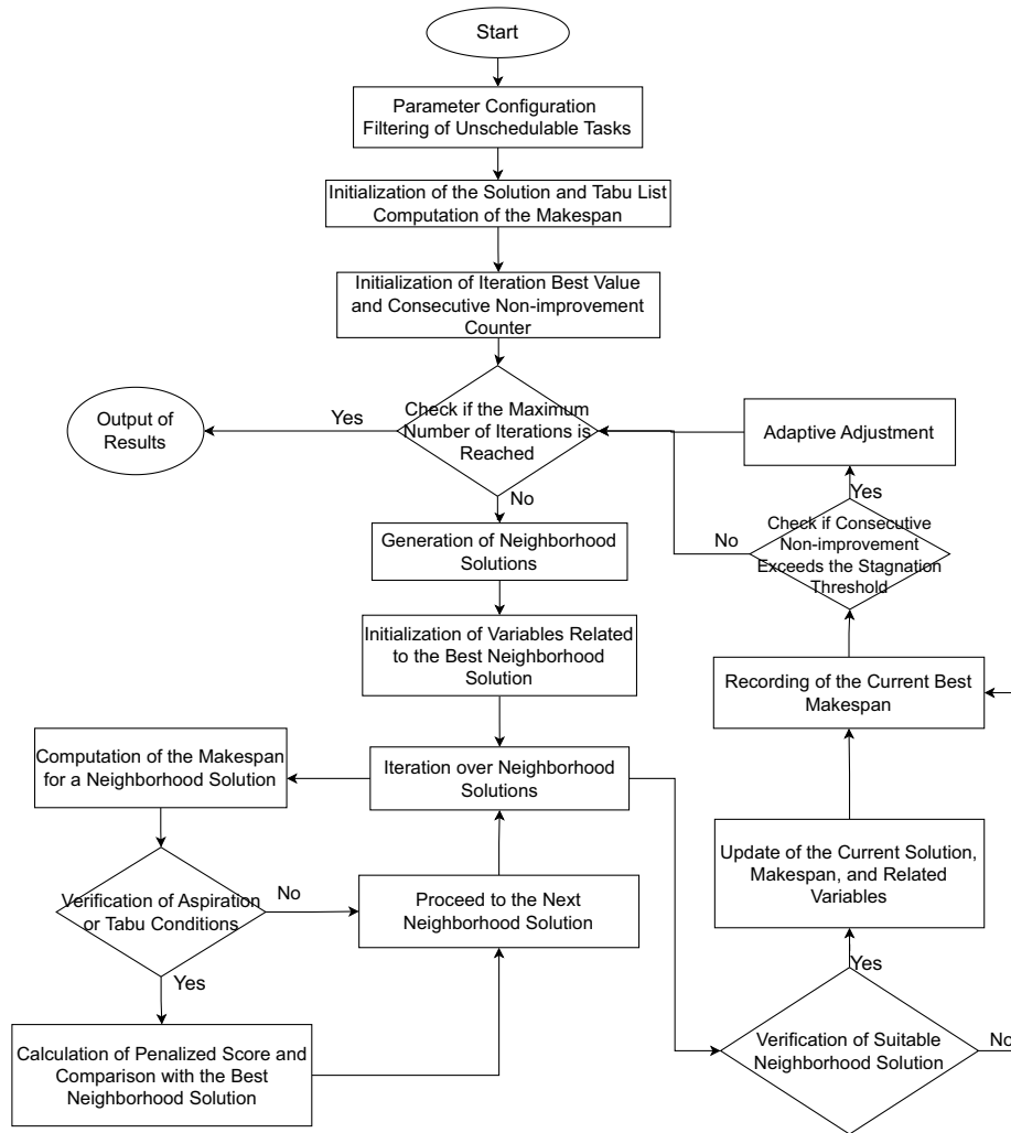
Fig. 1. Flowchart of the improved tabu search algorithm.
