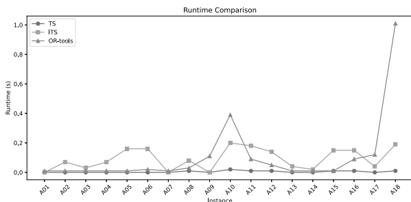
(b) runtime comparison on small-scale instances.
