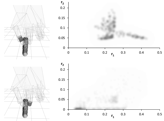
Fig. 3. Contact models by Kopicki et al. (2015). Left: a “pinch” training grasp with selected hand-links (dark grey), right: distributions of curvature descriptors r for features in each link’s contact model.
