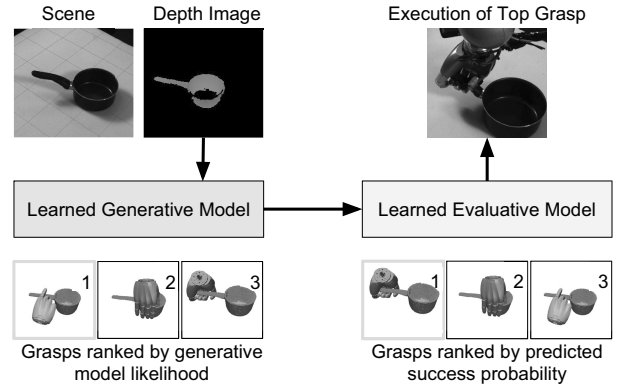
Fig. 13. Basic architecture of a generative-evaluative learner.
