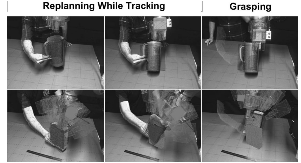
Fig. 15. Grasp adaptation examples. As objects move, grasp candidates are updated. The active grasp and next-best candidate are highlighted. The final column presents successful grasps.
