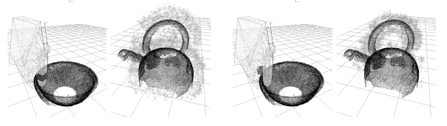
Fig. 7. Visualisation of two query densities (right image in each panel) for two contact models (left image in each panel) of a “pinch with support” grasp (Kopicki et al. , 2015). The links to which the contact models are associated are in dark grey. A query density is a distribution over poses of the corresponding link (light grey cloud) for a new query kettle.
