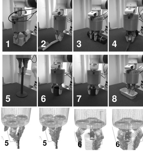
Fig. 12. Training examples 1–8 (top and middle rows), estimated and optimised contact models for training examples 5 and 6 (bottom row).
