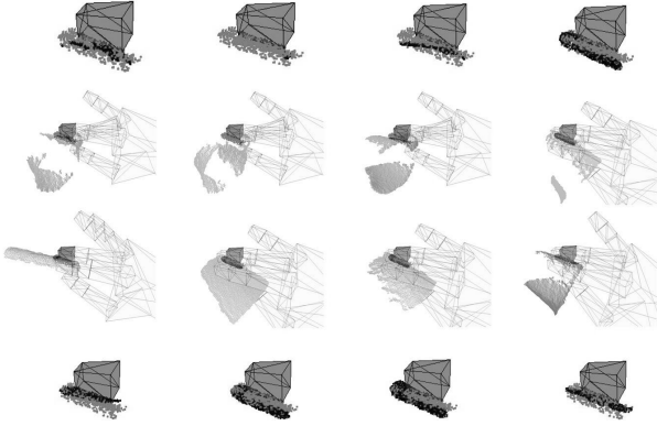
Fig. 5. Cluster members and point cloud data for one contact type (Kopicki et al. , 2019). Prototype (dark grey), members (black), hand-link (light grey).
