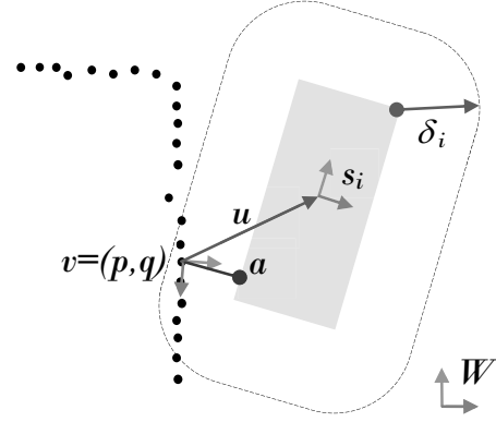
Fig. 2. Illustration of the contact receptive field F_i for hand-link i (light grey), showing surface samples (black dots), cutoff boundary \delta_i (black oval), and relative pose u .
