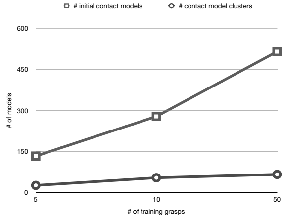
Fig. 8. Number of contact models before and after compression as the number of training grasps rises.
