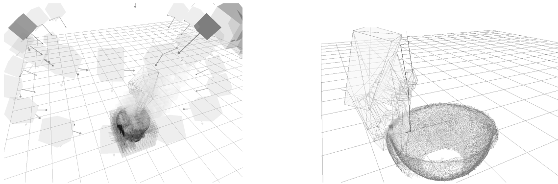
Fig. 16. Left: candidate camera poses \Xi , with visited poses V in darker grey; the voxel cube around the object is sculpted via information gain when no contacts are found. Right: example grasp with shaded contact regions; Active vision selects views to improve reconstruction at predicted contact sites.
