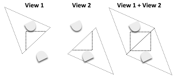
Fig. 1. Two-fingered grasp of an object, shown in cross-section. Object view models can be created from partial point clouds captured from single-camera view points (View 1 or View 2), but also from point clouds combined from multiple views (far right figure).
