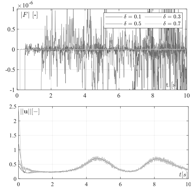
Fig. 8. Time-plots of positional errors in a linear scale (upper plot) and the corresponding plot of a control-vector norm illustrating an increase in closed-loop robustness to external high-frequency perturbation (HFP) \mu(t) by selecting a larger value of parameter \delta .
