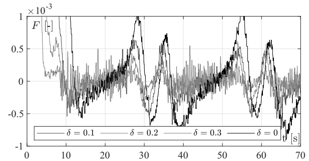
Fig. 12. Comparative experimental results of positional error evolution illustrating an increase in closed-loop robustness achievable for larger values of parameter \delta relative to the case of infinitely convergent control version corresponding to \delta = 0 .
