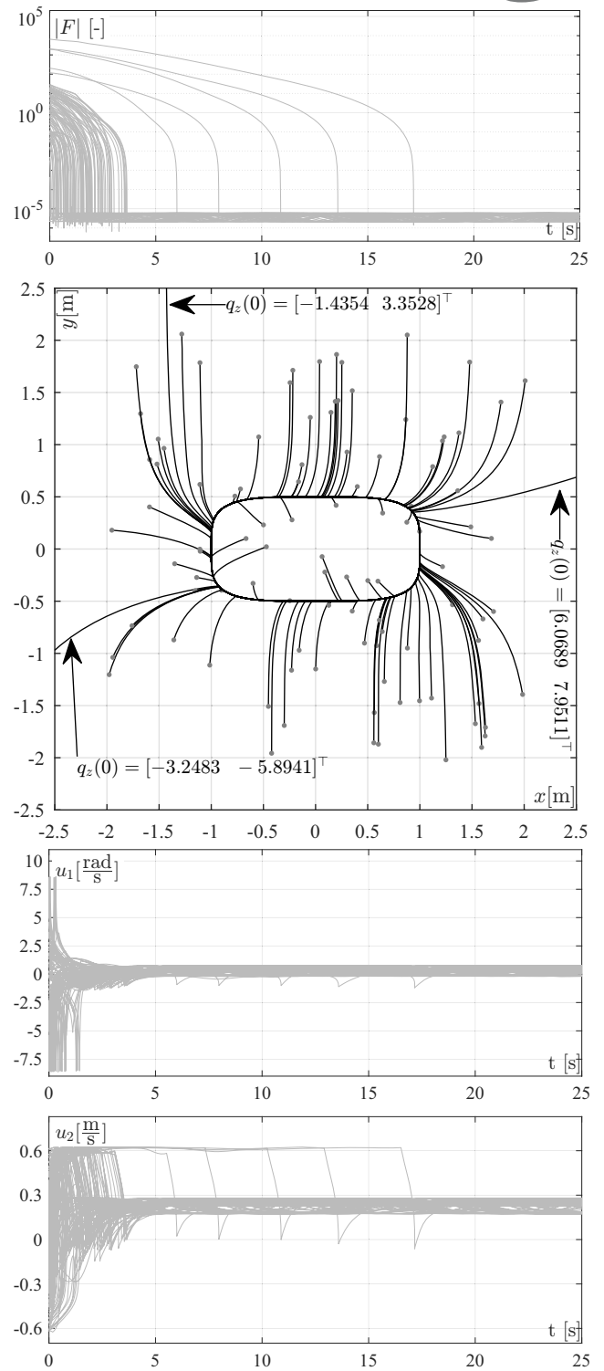
Fig. 5. Time evolution of positional absolute errors and a set of paths drawn by the robot's point Z when starting from various initial conditions (close to and far from the reference path), complemented with the corresponding time plots of control signals: the case for \delta = 0.7 .
