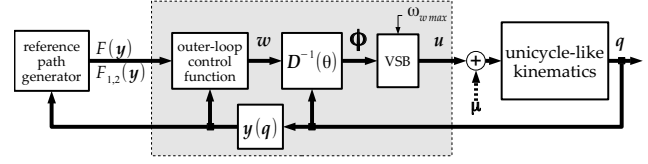
Fig. 2. Block scheme of the proposed positional control system for the unicycle-like kinematics (VSB: velocity scaling block; see the formulas (4)–(5)).
