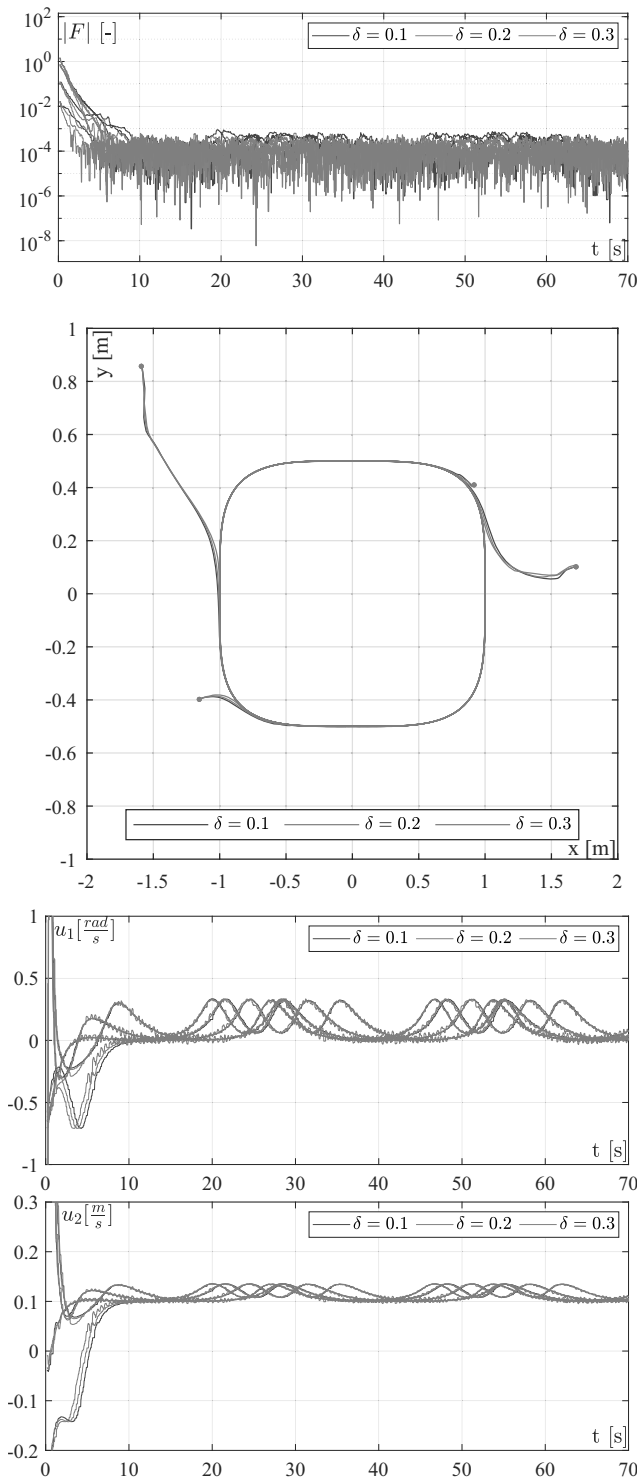
Fig. 11. Collection of comparative experimental results illustrating time evolutions of positional absolute errors and a set of paths drawn by MTracker's point Z when starting from four different initial conditions (denoted by the dots in the XY plot), complemented with the corresponding time plots of control signals for three selected values of parameter \delta .
