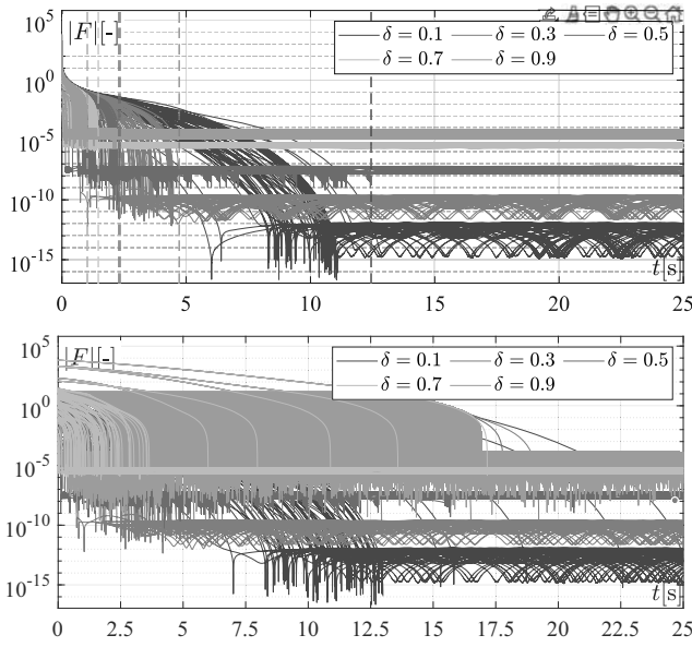
Fig. 6. Absolute positional errors in a logarithmic scale for various values of parameter \delta obtained for a set of 70 randomly selected initial robots configurations in the control-unconstrained case (upper plot) and in the control-constrained case (bottom plot).
