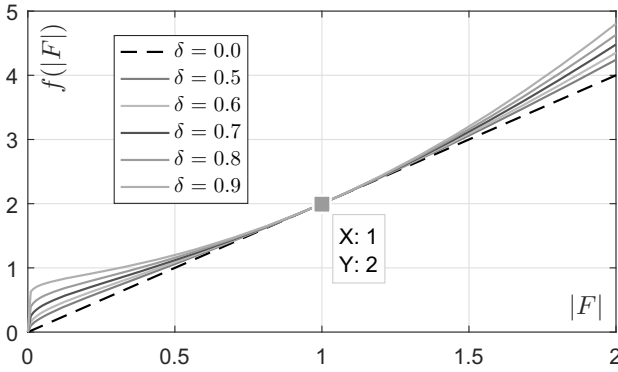
Fig. 3. Plots of function f(|F|) = |F|^{1+\delta} + |F|^{1-\delta} for various values of parameter \delta (together with the limit case for \delta = 0 , included for better reference); point (|F|, f(|F|)) = (1, 2) is common for all the plots.
