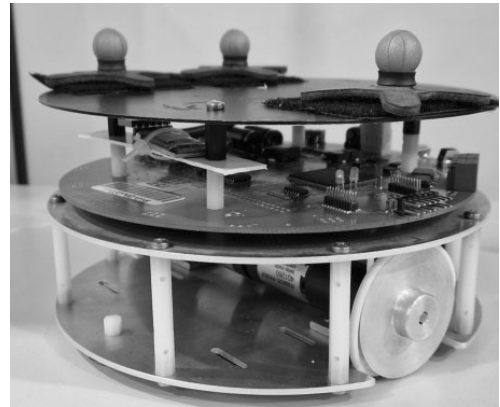
Fig. 10. Experimental laboratory-scale differentially driven robot MTracker built in the Institute of Automatic Control and Robotics of the PUT.
