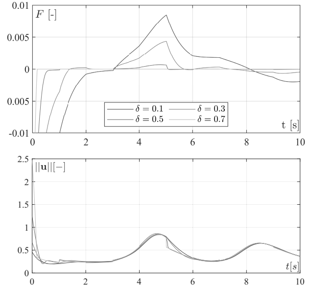
Fig. 7. Time-plots of positional errors in a linear scale (upper plot) and the corresponding plot of a control-vector norm illustrating an increase in closed-loop robustness to external low-frequency perturbation (LFP) \mu(t) by selecting a larger value of parameter \delta .
