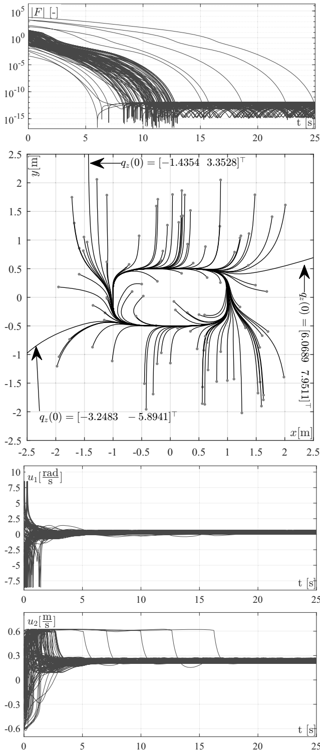
Fig. 4. Time evolution of positional absolute errors and a set of paths drawn by the robot's point Z when starting from various initial conditions (close to and far from the reference path), complemented with the corresponding time plots of control signals: the case for \delta = 0.1 .
