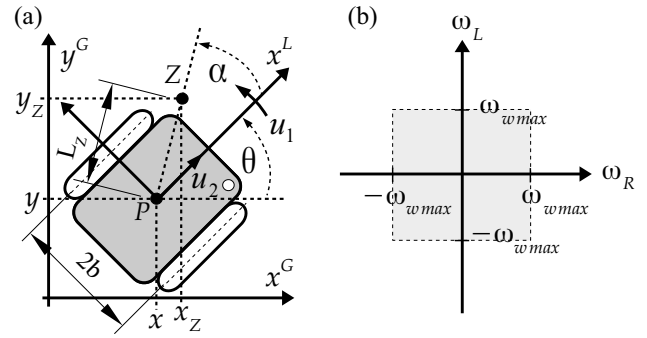
Fig. 1. Kinematics of the unicycle-like mobile robot with a definition of point Z (a), a set of the admissible robot's wheel speeds which determines the constrained set \mathcal{U} of the robot's control inputs (b).
