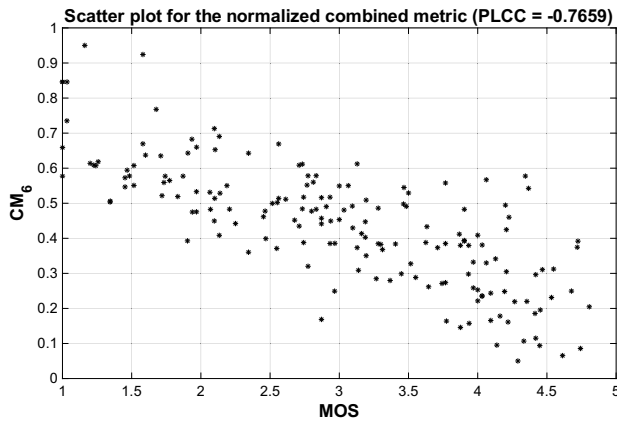
Fig. 10. Scatter plot obtained for the normalized combined metric constructed from six elementary metrics.
