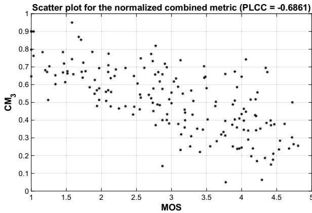
Fig. 7. Scatter plot obtained for the normalized combined metric constructed from three elementary metrics.
