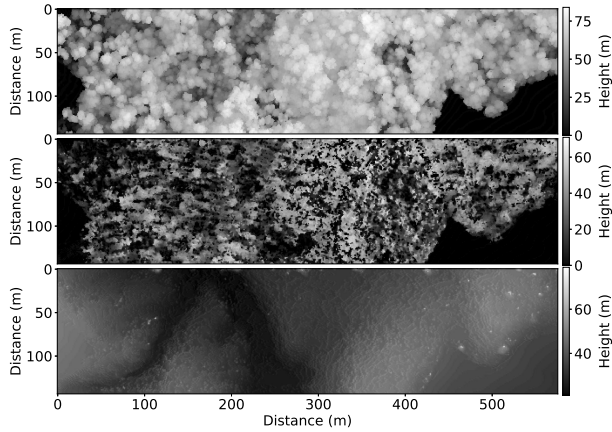
Fig. 1. HHDC-derived 2D products via percentile slicing. Top: canopy height model computed per footprint as \text{CHM}(i, j) = h_{98}(i, j) - h_2(i, j) , where h_p is the p -th percentile of the within-footprint vertical return distribution from the hyper-height data cube. Middle: median elevation map h_{50}(i, j) , summarizing the central tendency of the canopy/understory structure and often used as a biomass proxy. Bottom: digital terrain model estimated from the 2nd percentile h_2(i, j) , approximating the bare-Earth surface.
