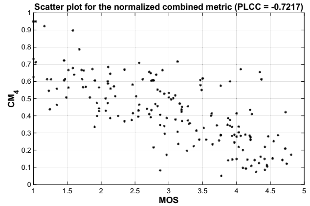
Fig. 8. Scatter plot obtained for the normalized combined metric constructed from four elementary metrics.
