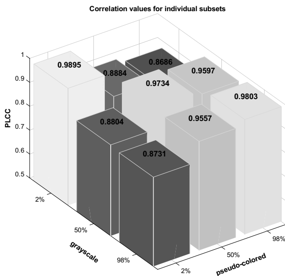
Fig. 4. PLCC values between the grayscale and pseudo-colored images representing individual percentiles.
