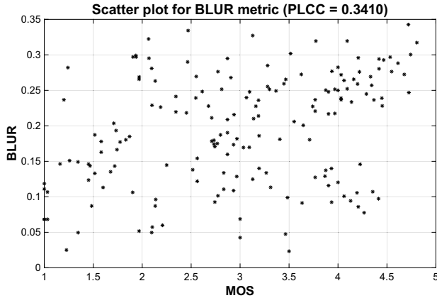
Fig. 5. Scatter plot obtained for the elementary metric demonstrating the highest correlation with MOS values.
