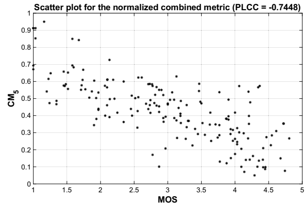
Fig. 9. Scatter plot obtained for the normalized combined metric constructed from five elementary metrics.
