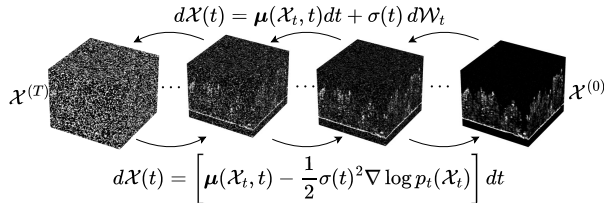
Fig. 2. Diffusion generative model for estimating p(\mathcal{X}) . The forward process (top) uses an SDE to add noise to clean data \mathcal{X}(0) , shown as cubes transitioning from structured to noisy states. The reverse process (bottom), guided by a probability flow ODE and a neural network-estimated score, denoises \mathcal{X}(T) back to \mathcal{X}(0) .
