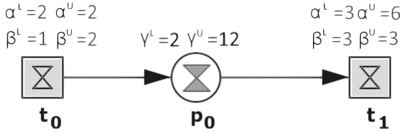
Fig. 1. Extended time Petri net with time intervals \alpha and \beta assigned to transitions and time interval \gamma assigned to a place.
