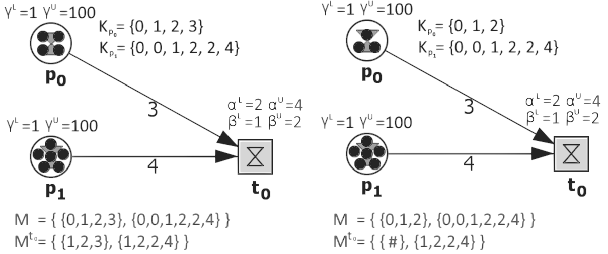
Fig. 2. Example of conditions when a transition is active or inactive.
