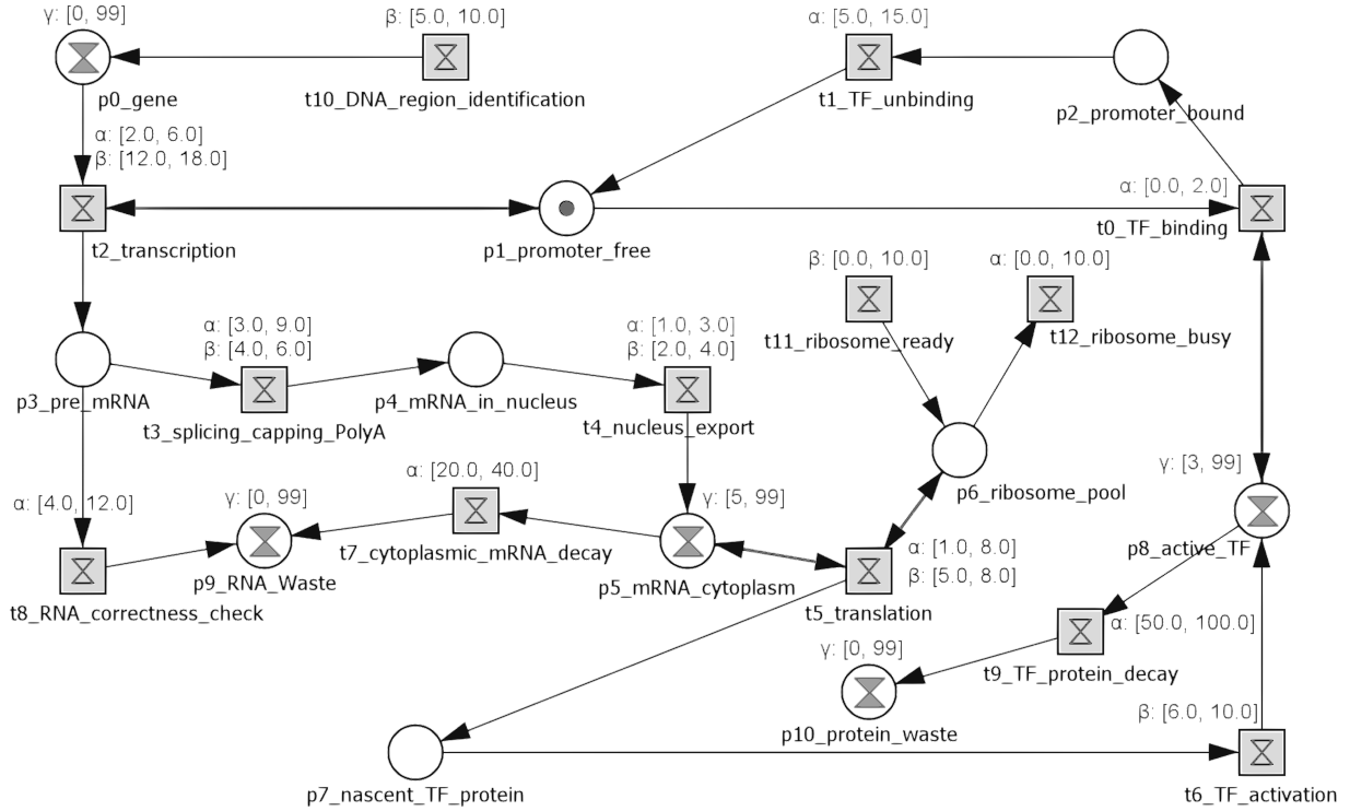
Fig. 3. Example model of gene expression with negative transcription feedback. Places and transitions are annotated with their timing parameters. Circles without hourglasses represent places without time constraints.
