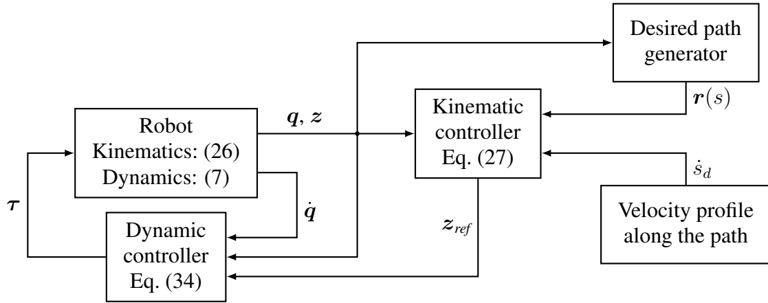
Fig. 3. General scheme of the cascade control structure.
