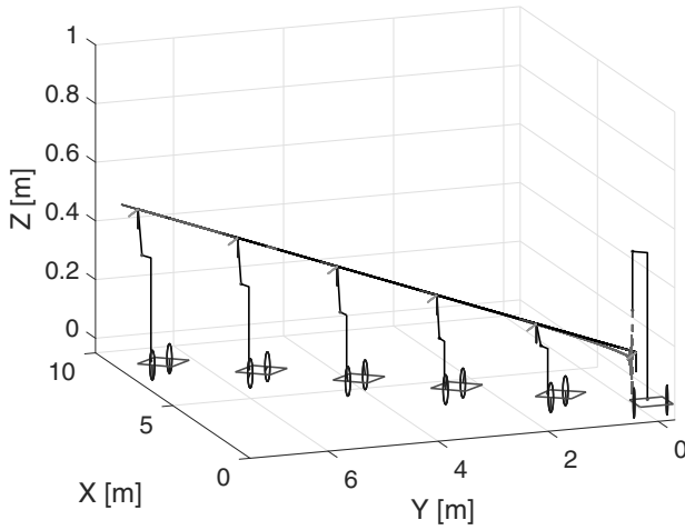
Fig. 5. Path followed by the mobile manipulator.
