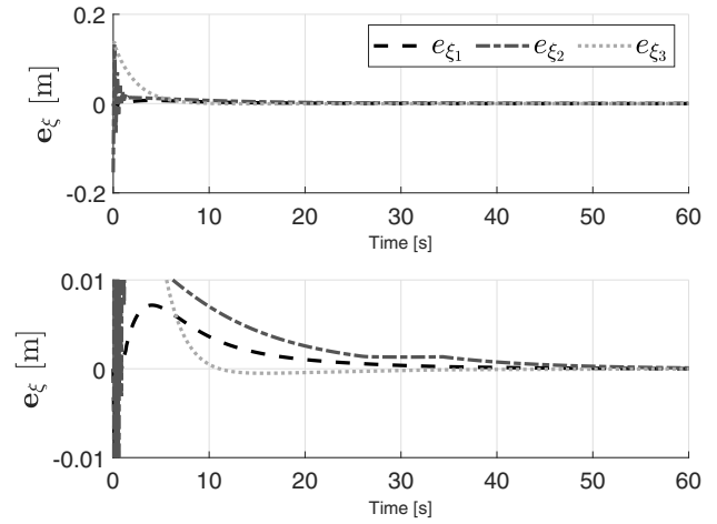
Fig. 6. Path following errors.
