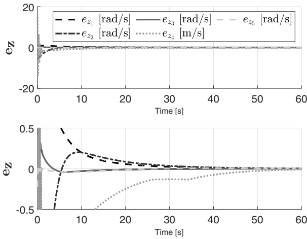
Fig. 7. Velocity profile following errors.
