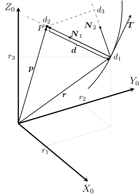
Fig. 1. Orthogonal projection of an object onto a curve.
