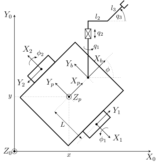
Fig. 4. Schematic view of the mobile manipulator.
