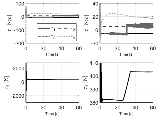
Fig. 8. Control signals.
