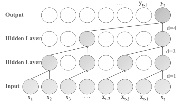
Fig. 5. Dilated convolution.
