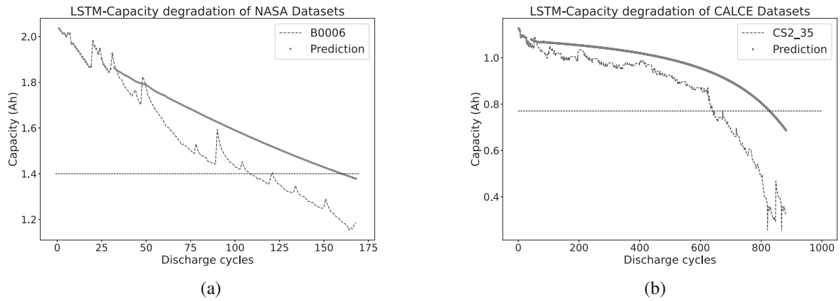
Fig. 12. RUL prediction fitting effect of the LSTM network: NASA dataset (a), CALCE dataset (b).
