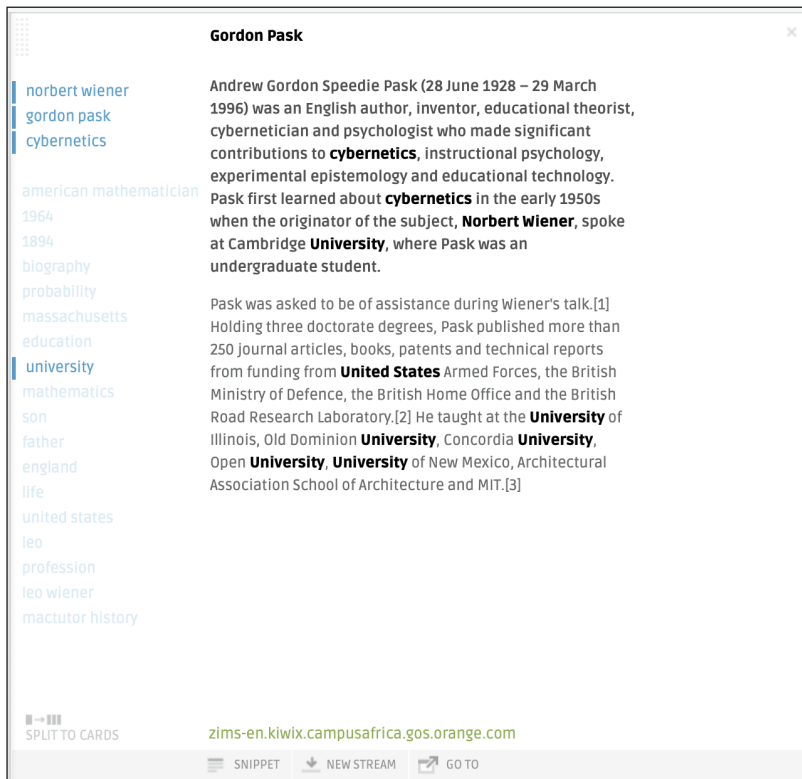
Figure 10 Parsed information.
