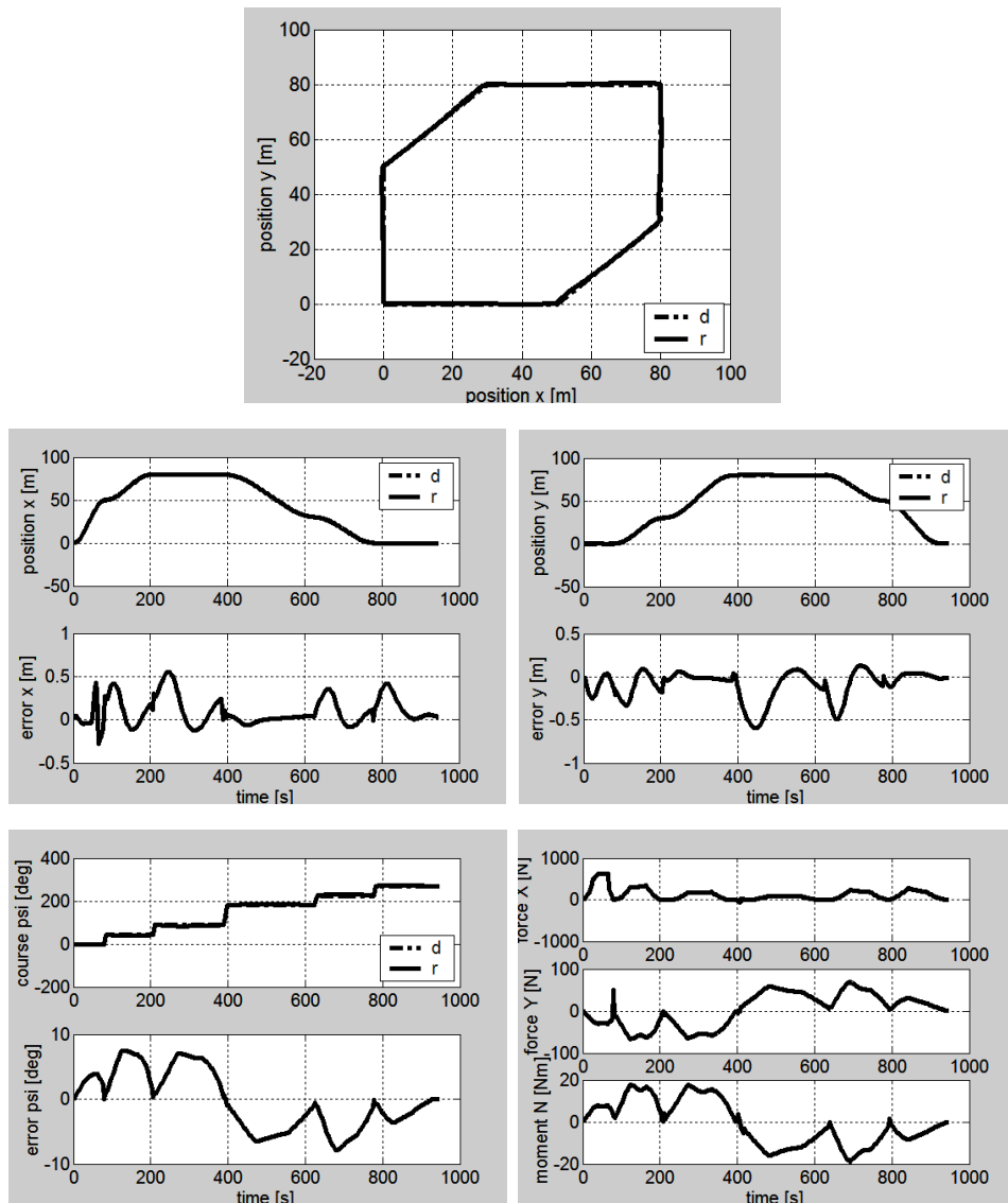
Fig. 3. Track-keeping control under interaction of sea current disturbances (average velocity 0.3 m/s and direction 135^\circ ): desired (d) and real (r) trajectories (upper plot), x-, y-position and error of position (middle plots), course and its error and commands (low plots) [own work]
