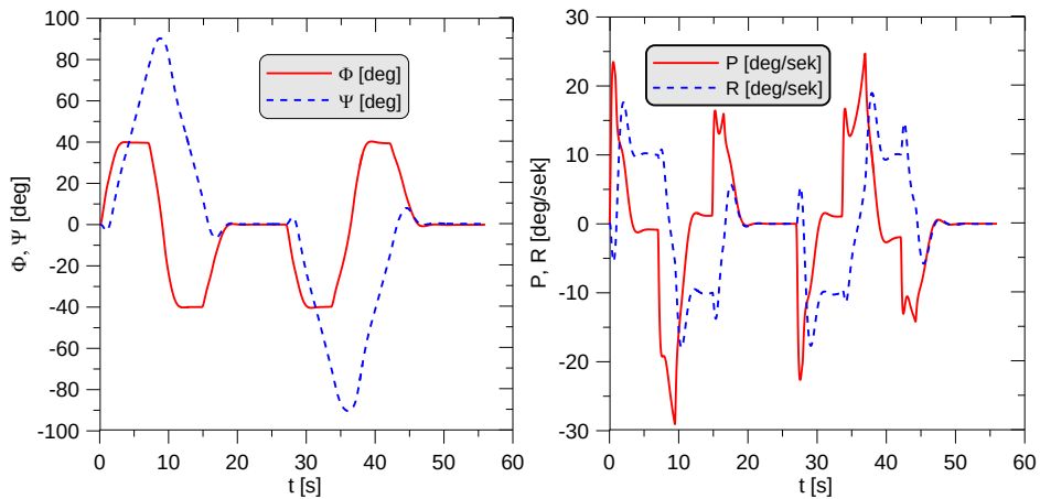
Fig. 4a, 4b. Angles and the appropriate angular velocities for roll and yaw motion (flaps deflected) [own work]
