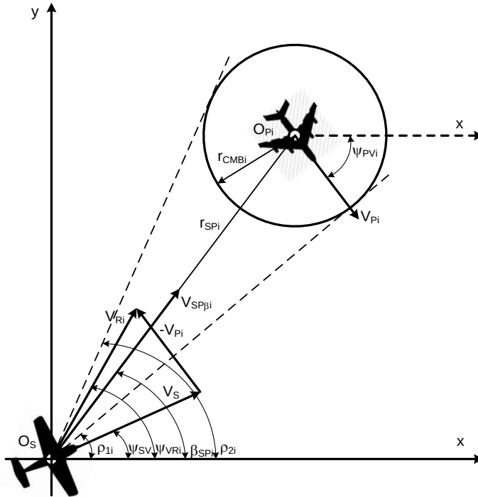
Fig. 3. Variables describing the aircraft — obstacle configuration [own work]
