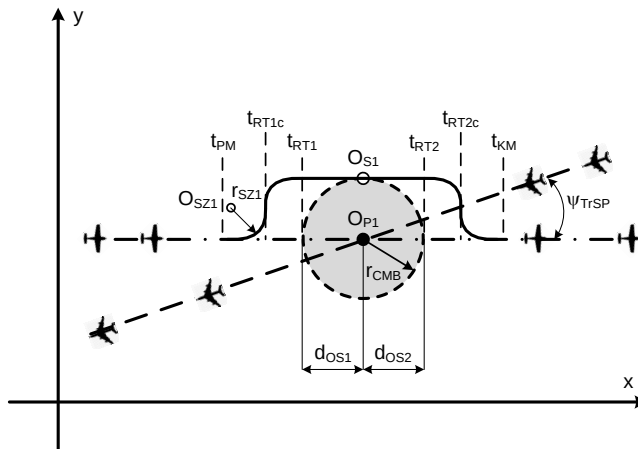
Fig. 1. The proposed trajectory of evasive manoeuvre [own work]
