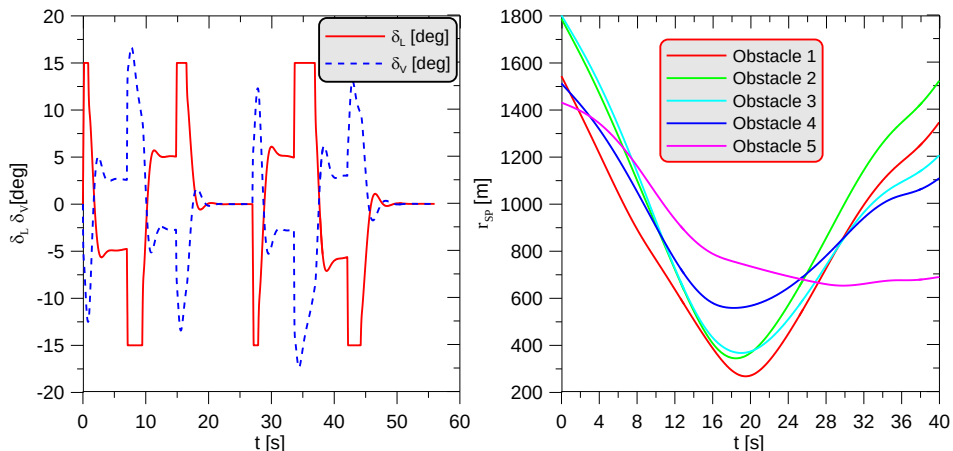
Fig. 5a, 5b. Ailerons and ruder deflections and airplane — to-obstacle distance (flaps deflected) [own work]
