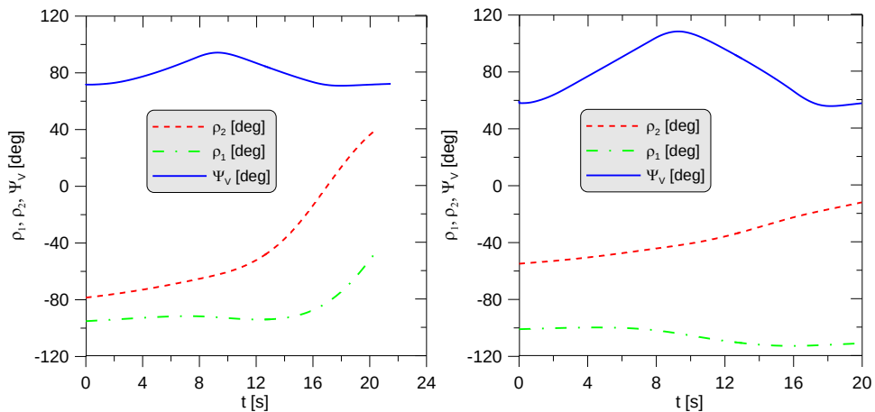
Fig. 7a, 7b. The angles of tangents to the circle of radius r_{CMBi} and the angle of resultant velocity vector of the airplane and obstacles No. 3 and No. 5 [own work]
