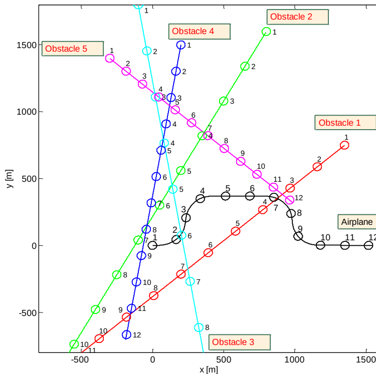
Fig. 8. Trajectories of the airplane and moving obstacles obtained by simulation [own work]
