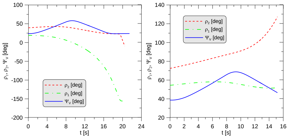
Fig. 6a, 6b. The angles of tangents to the circle of radius r_{CMBi} and the angle of resultant velocity vector of the airplane and obstacles No. 1 and No. 2 [own work]
