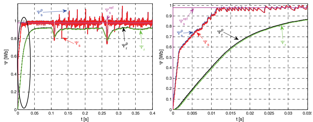
Fig. 8. Waveforms of fluxes ( \Omega = 0.25\Omega_N )
