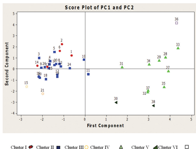
Figure 2. Score plot of PC1 and PC2 for 38 chilli genotypes
