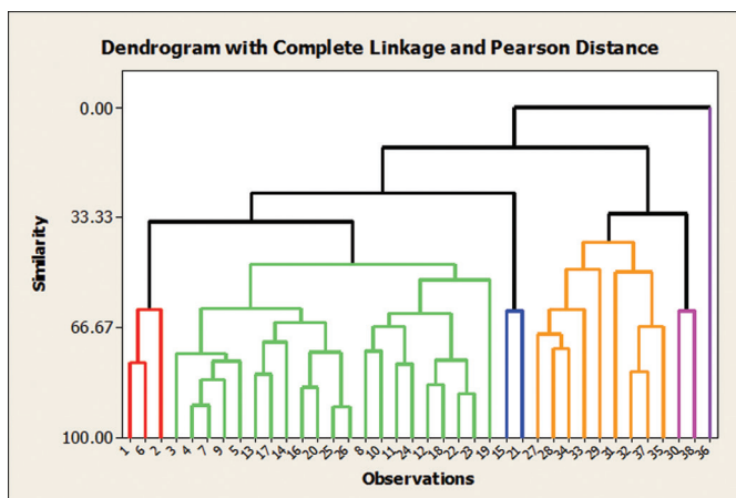
Figure1. Dendrogram based on 14 morphological characters in 38 chilli genotypes
