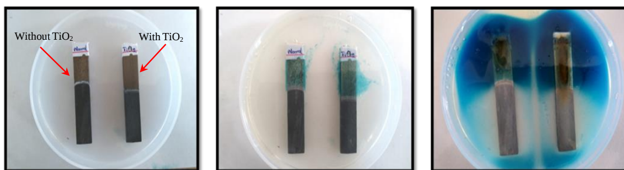
Fig. 4. Progression of the corrosion with the FerroxyI reagent test. (a) Before the test, (b) after five minutes, and (c) after 24 hours of starting the test.
