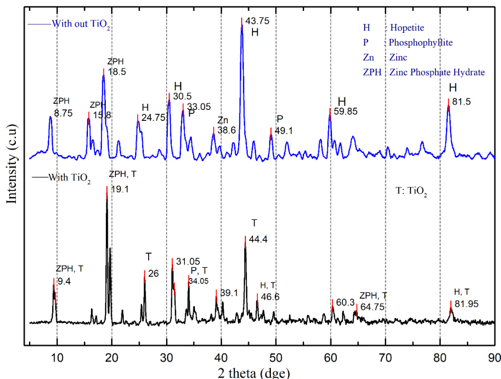
Fig. 3. XRD patterns of the phosphate coating on mild steel substrate, (a) without \text{TiO}_2 , and (b) with \text{TiO}_2 .
