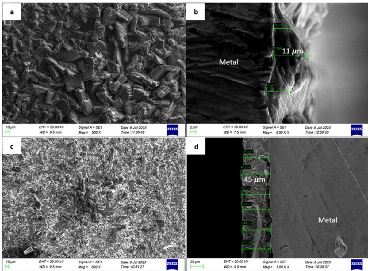
Fig. 2. (a) and (b) exhibits the SEM images of phosphate coating on mild steel without \text{TiO}_2 , (magnification 500x and 4500x, respectively). (c) and (d) exhibits the SEM images of phosphate coating on mild steel with \text{TiO}_2 , (magnification 500x and 1000x, respectively). Thicknesses of the coating layers are shown with horizontal bars drawn in cross sectional SEM images of (b) and (d).
