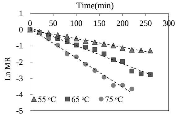
Fig 9. \ln(MR) vs time at different temperatures for black pepper dried in a fluidized bed dryer at different drying temperatures.; Experiment conditions: U_{\text{mf}} = 8 \text{ m/s} , M_{\text{io}} = 325 \% , bed weight = 0.75 kg
