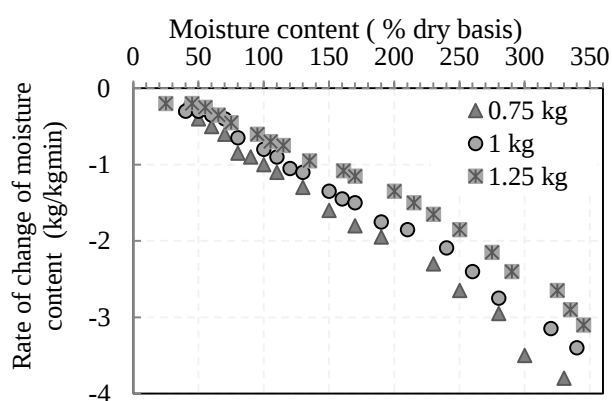
Fig 6. Rate of change of moisture content ( dm/dt ) versus moisture content (% dry basis) at three different bed weights of black pepper when dried in fluidized bed dryer; Experiment conditions: M_{i0} = 325\% , T = 65^\circ\text{C} , U_{mf} = 8\text{ m/s} , 9.5\text{ m/s} and 11\text{ m/s} for bed weights 0.75\text{ kg} , 1\text{ kg} and 1.25\text{ kg} respectively
