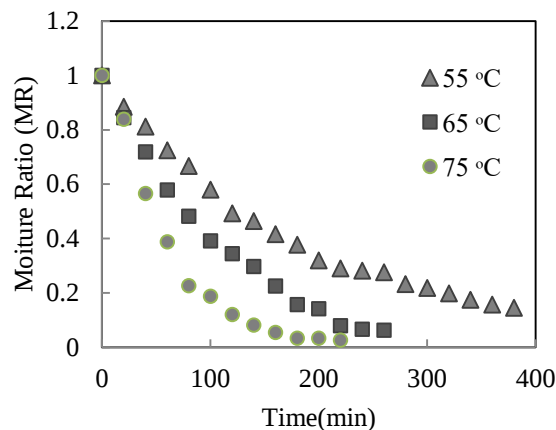
Fig 7. Moisture ratio versus time at different temperatures for black pepper when dried in fluidized bed dryer at different drying temperatures; Experiment conditions: U_{mf} = 8\text{ m/s} , M_{i0} = 325\% , bed weight = 0.75\text{ kg}
