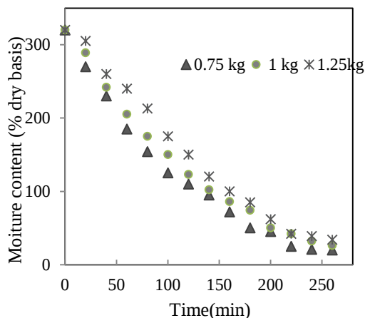
Fig 5. Moisture content (% dry basis) versus time at three different bed weights of black pepper when dried in fluidized bed dryer; Experiment conditions: M_{i0} = 325\% , T = 65^\circ\text{C} , U_{mf} = 8\text{ m/s} , 9.5\text{ m/s} and 11\text{ m/s} for bed weights 0.75\text{ kg} , 1\text{ kg} and 1.25\text{ kg} respectively.
