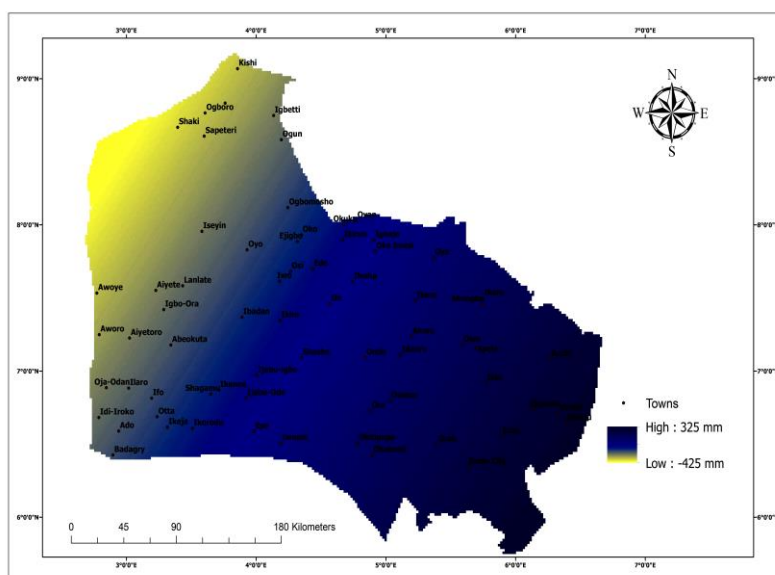
Fig. 7. Mean annual pattern of water balance in the study area (1976-2015).
