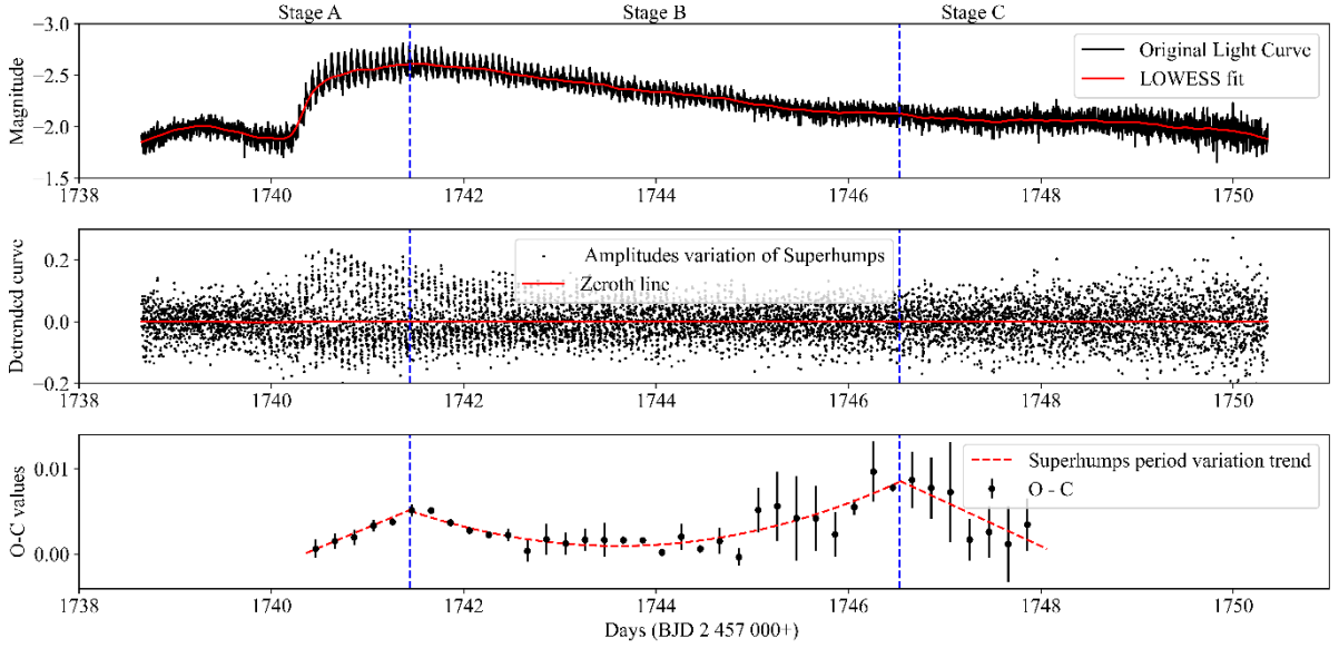
Figure 2c: Top panel shows the light curve of superoutburst of IX Dra (Sector 16). Middle panel shows the detrended light curve. Bottom panel shows the O-C diagram of the superhumps.
