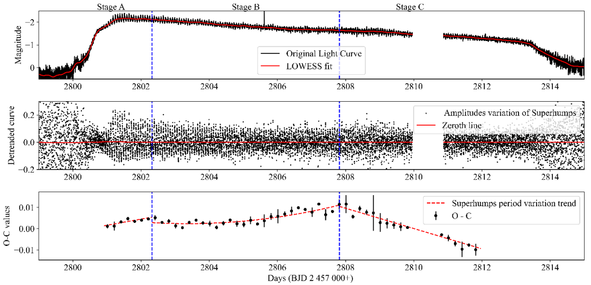
Figure 2f: Top panel shows the light curve of superoutburst of IX Dra (Sector 55). Middle panel shows the detrended light curve. Bottom panel shows the O-C diagram of the superhumps.
