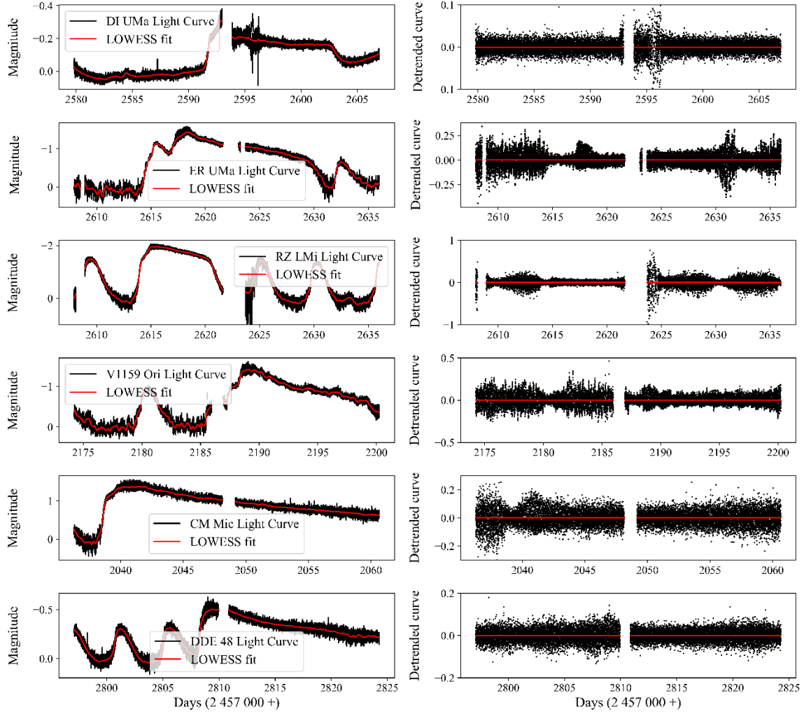
Figure 1a: The left panels show light curves of the superoutbursts of DI UMa, ER-UMa, RZ LMi, V1159 Ori, CM Mic and DDE48. The right panels show detrended light curves of those stars respectively.
