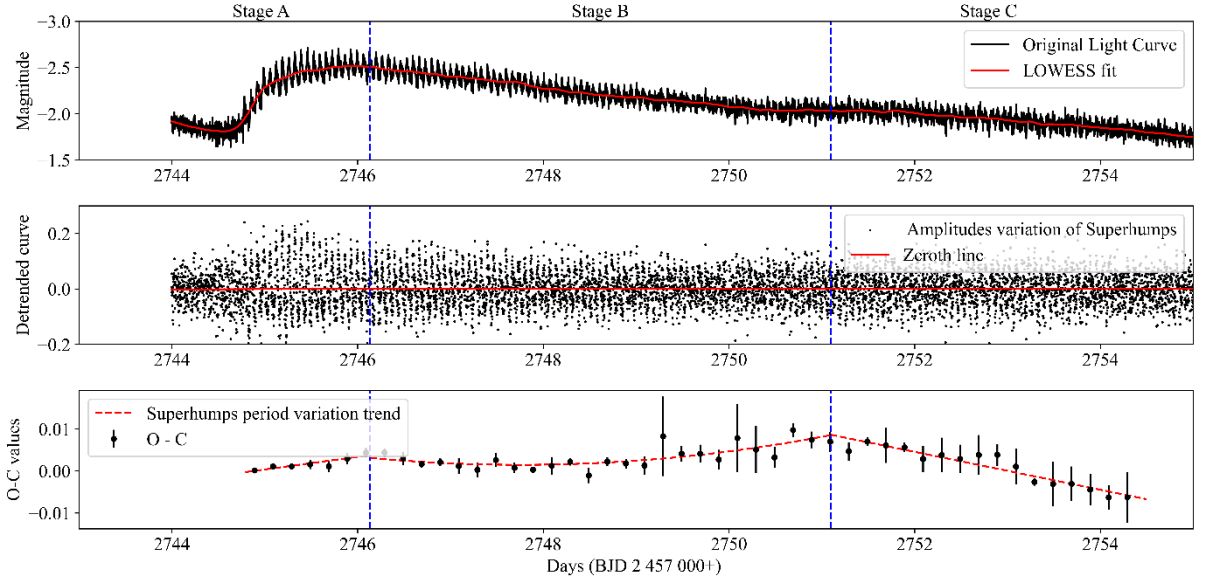
Figure 2e: Top panel shows the light curve of superoutburst of IX Dra (Sector 53). Middle panel shows the detrended light curve. Bottom panel shows the O-C diagram of the superhumps.
