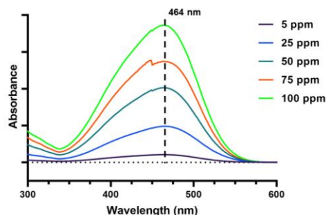
Figure 1. UV-Vis spectrum of the MO at different concentration
