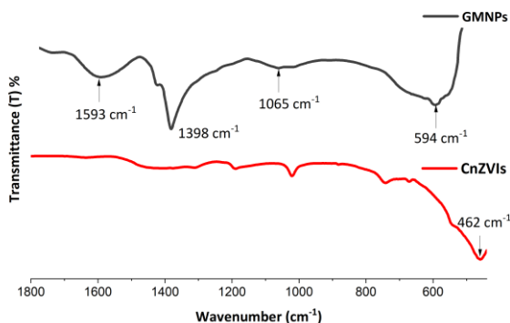
Figure 2. FT-IR spectrums of the GMNPs and CnZVIs
