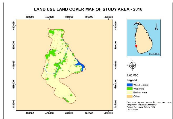
Figure 11: Land Use Land Cover map of the study area in 2016
