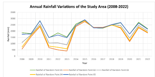
Figure 16: Annual Rainfall Variation of Study Area
