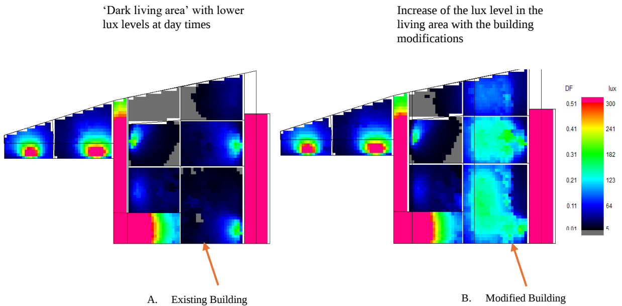
Fig 11. Daylight Conditions
