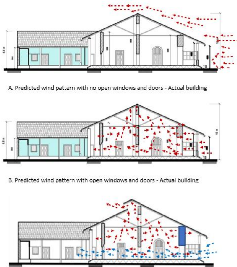
Fig. 6. Predicted wind patterns according to the air-fluid dynamic principles (stack effect and stack-induced ventilation )
