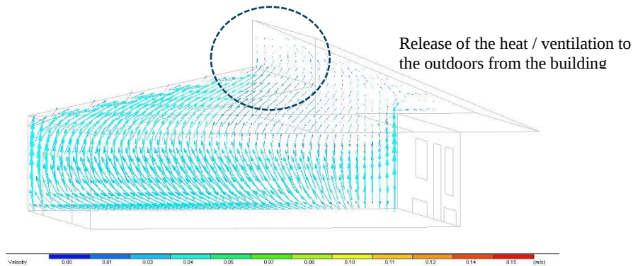
Fig. 10. Air flow pattern after modifying the building with upper and
