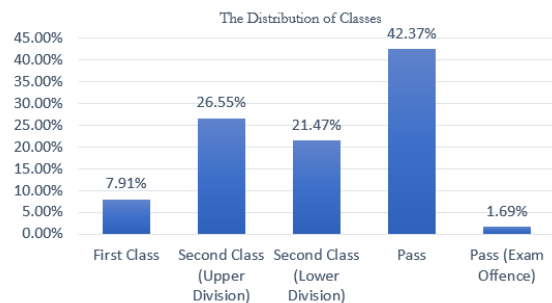
Figure 20: Class Distribution
