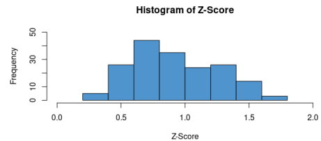
Figure 1: Histogram of Z-Score
