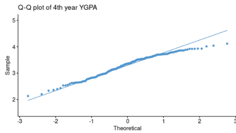
Figure 18: Normal Q-Q plot of 4 th year YGPA
