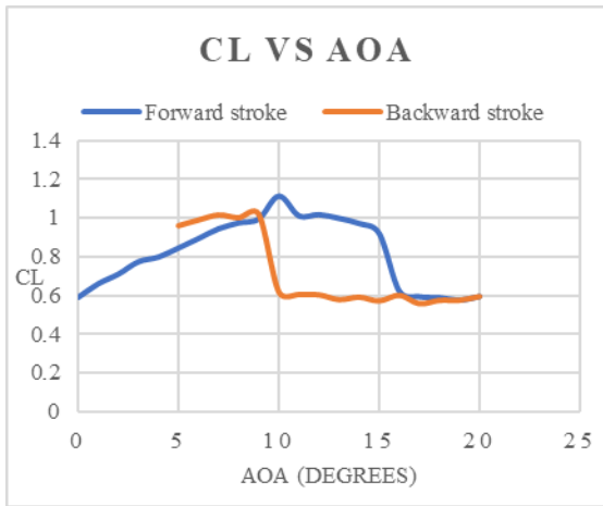
Figure 6. CL variation for forward and backward stroke at Reynolds number of 134072
