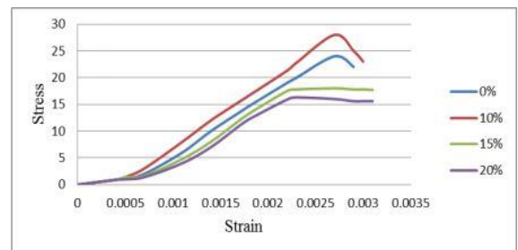
Figure 2.1: Relationship between stress and strain for different crumb rubber percentages in concrete (Dass and Sharma, 2013)
