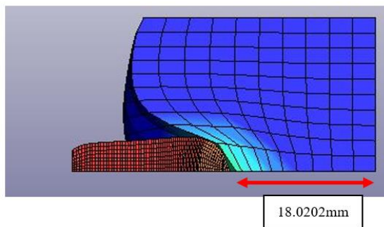
Figure 4.2: Rubberized Concrete Deformed Shape of the Model after the Impact under 300\text{ms}^{-1} Projectile Velocity
