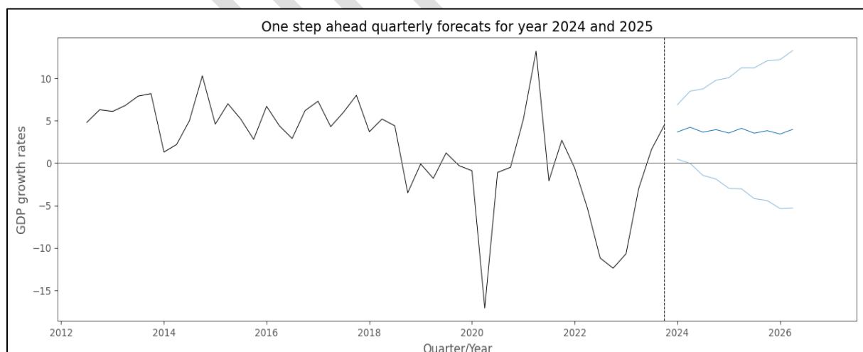
Figure 4. Fitted and Forecasts of GDP Growth Rates Using Fitted Harvey-Type STM Model
