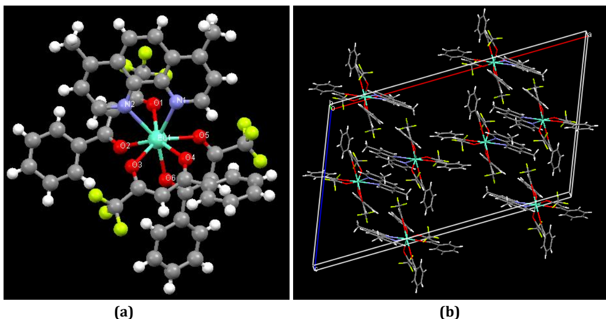
Figure 3. (a) Single crystal X-ray crystal structure and (b) the unit cell packing diagram of \text{Eu}(\text{btfa})_3(\text{dmphen}) complex
