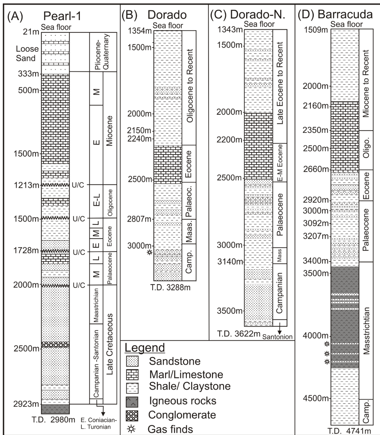
Fig. 2: Generalised stratigraphic sections of the wells (a) Pearl-1, (b) Dorado, (c) Dorado-North and (d) Barracuda (modified after Premaratne et al., 2015). Oligo. = Oligocene, Palaeoc. = Palaeocene, Maas. = Maastirchian, Camp. = Campanian, E = Early, M = Middle, L = Late, U/C = unconformity, and T.D. = total depth.
